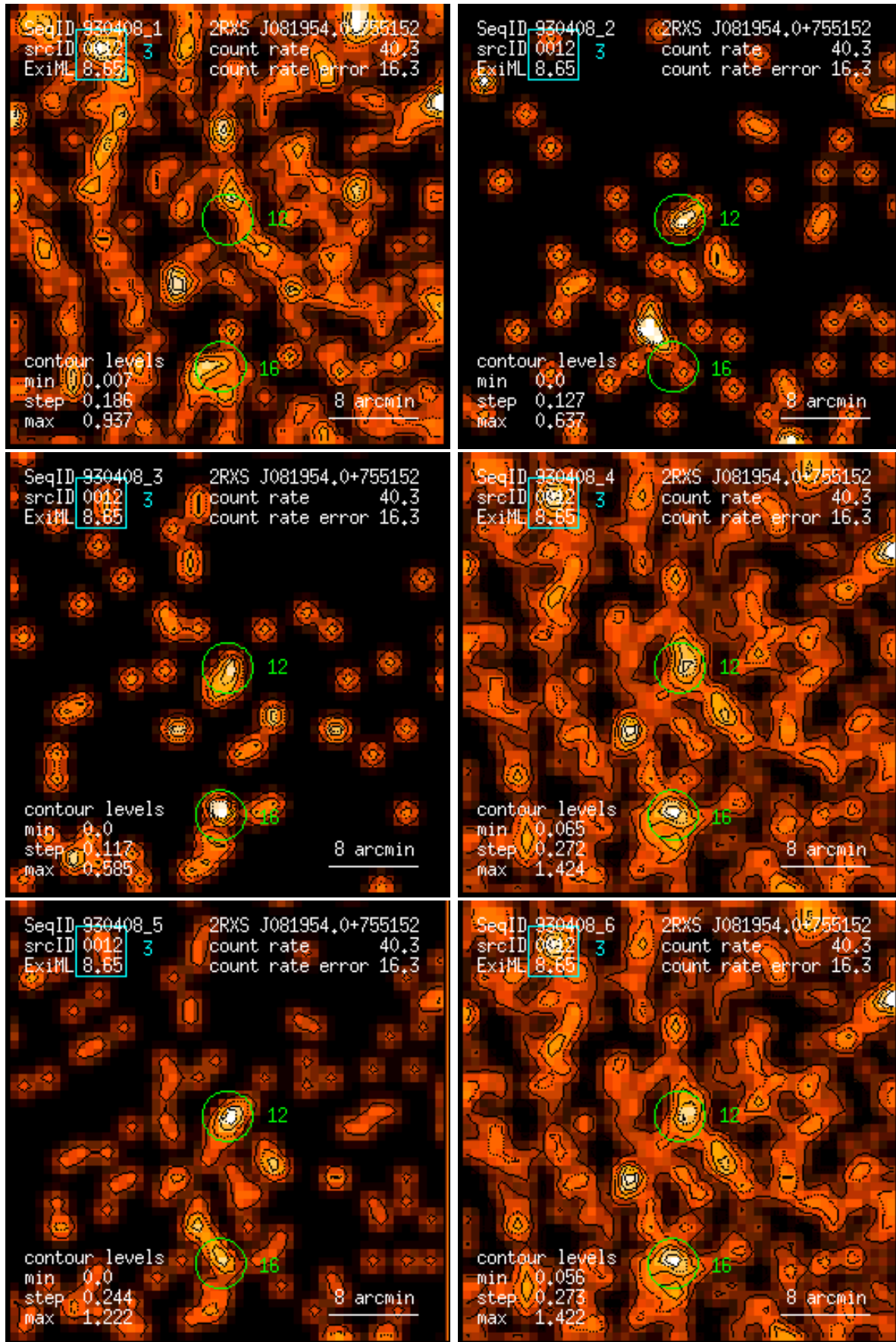
Figure 12: RASS 930408: detection 0012: band rate images, Gaussian filter: (1) PSPC channels 11 – 41, (2) 52 – 90, (3) 91 – 201, (4) 11 – 235, (5) 52 – 201, (6) 11 – 201. Broad band rates in counts/ks. Band rate contour levels in counts/ks/arcmin 2 .
