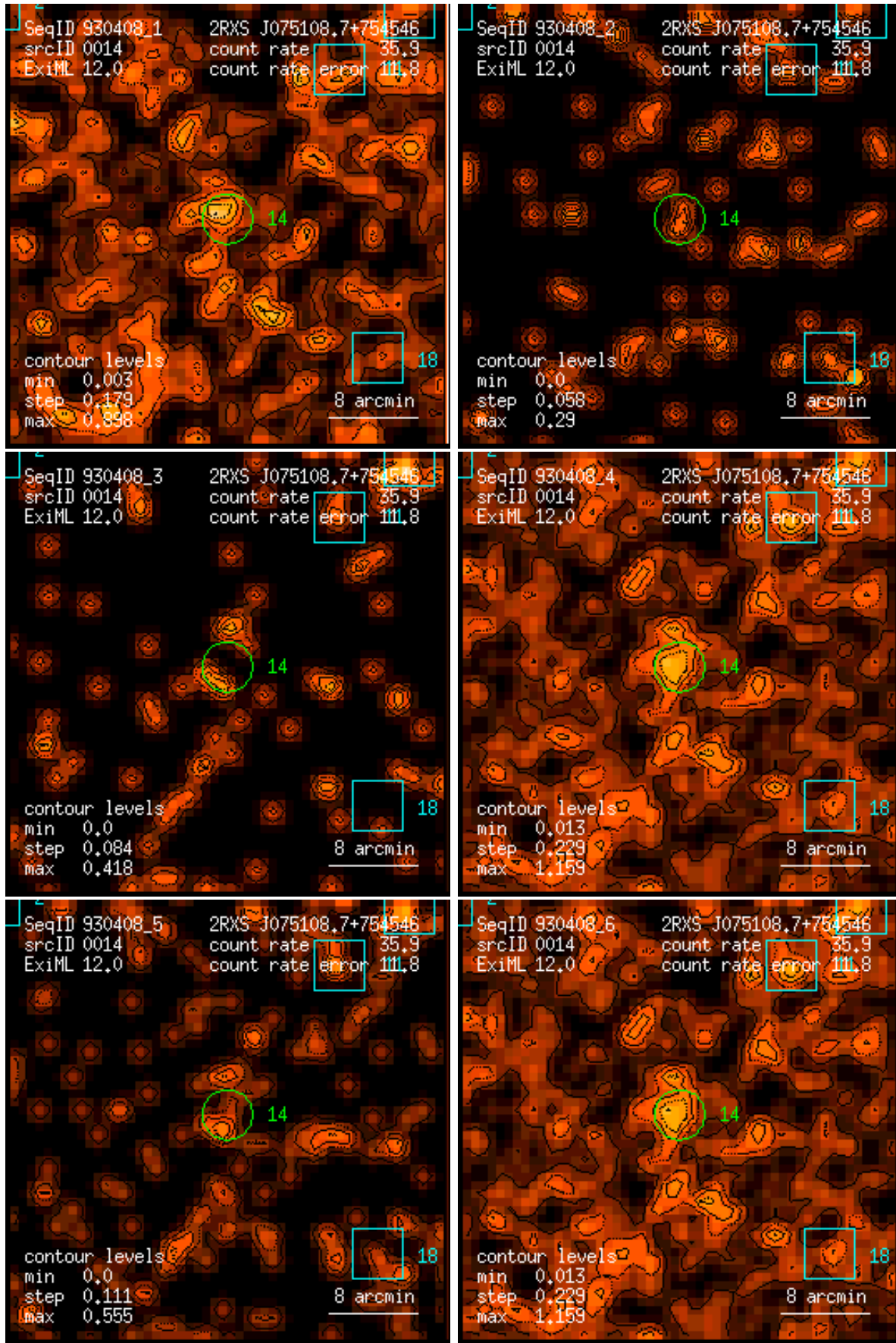
Figure 14: RASS 930408: detection 0014: band rate images, Gaussian filter: (1) PSPC channels 11 – 41, (2) 52 – 90, (3) 91 – 201, (4) 11 – 235, (5) 52 – 201, (6) 11 – 201. Broad band rates in counts/ks. Band rate contour levels in counts/ks/arcmin 2 .
