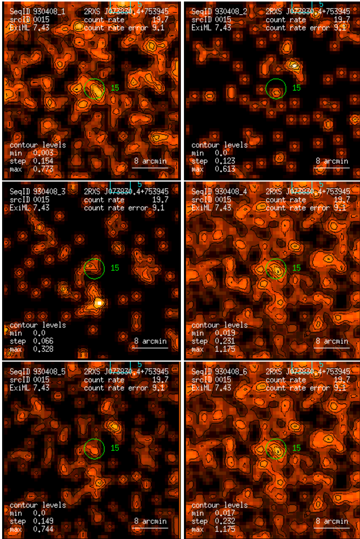
Figure 15: RASS 930408: detection 0015: band rate images, Gaussian filter: (1) PSPC channels 11 – 41, (2) 52 – 90, (3) 91 – 201, (4) 11 – 235, (5) 52 – 201, (6) 11 – 201. Broad band rates in counts/ks. Band rate contour levels in counts/ks/arcmin 2 .
