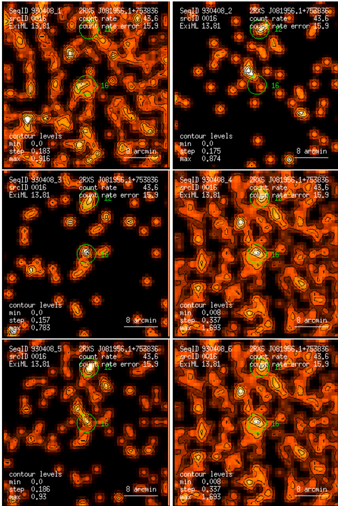
Figure 16: RASS 930408: detection 0016: band rate images, Gaussian filter: (1) PSPC channels 11 – 41, (2) 52 – 90, (3) 91 – 201, (4) 11 – 235, (5) 52 – 201, (6) 11 – 201. Broad band rates in counts/ks. Band rate contour levels in counts/ks/arcmin 2 .
