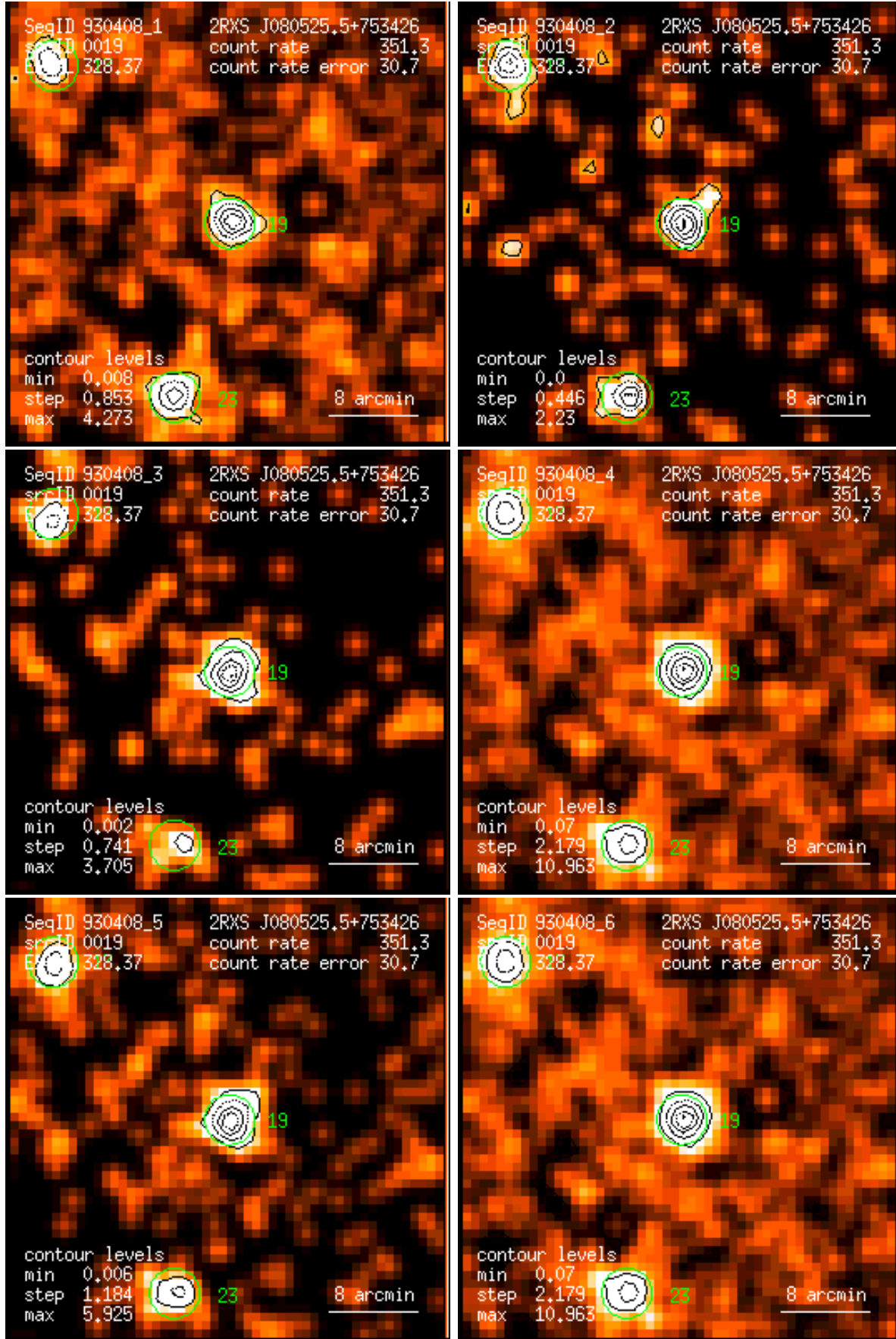
Figure 19: RASS 930408: detection 0019: band rate images, Gaussian filter: (1) PSPC channels 11 – 41, (2) 52 – 90, (3) 91 – 201, (4) 11 – 235, (5) 52 – 201, (6) 11 – 201. Broad band rates in counts/ks. Band rate contour levels in counts/ks/arcmin 2 .
