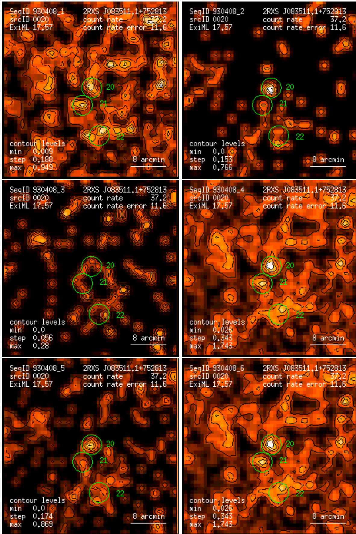
Figure 20: RASS 930408: detection 0020: band rate images, Gaussian filter: (1) PSPC channels 11 – 41, (2) 52 – 90, (3) 91 – 201, (4) 11 – 235, (5) 52 – 201, (6) 11 – 201. Broad band rates in counts/ks. Band rate contour levels in counts/ks/arcmin 2 .
