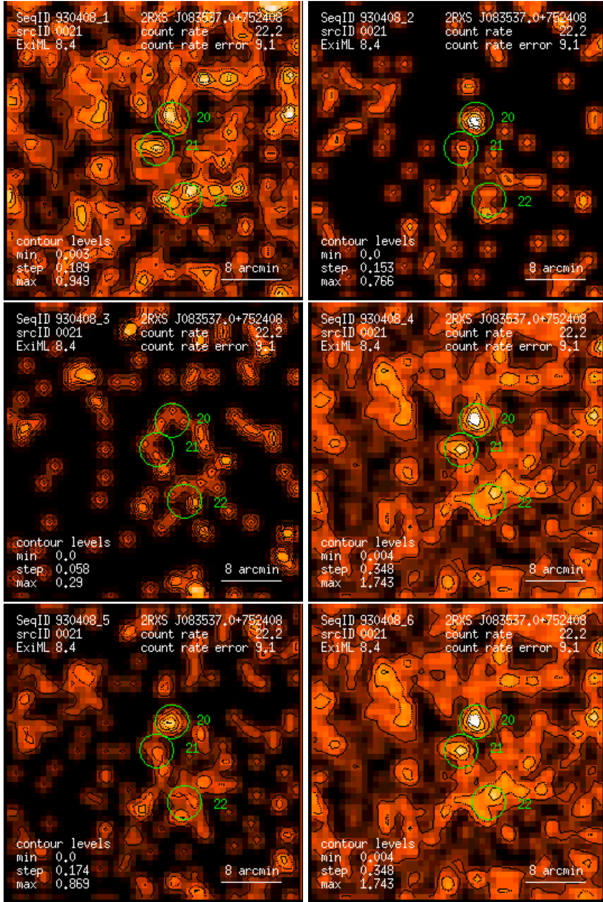
Figure 21: RASS 930408: detection 0021: band rate images, Gaussian filter: (1) PSPC channels 11 – 41, (2) 52 – 90, (3) 91 – 201, (4) 11 – 235, (5) 52 – 201, (6) 11 – 201. Broad band rates in counts/ks. Band rate contour levels in counts/ks/arcmin 2 .
