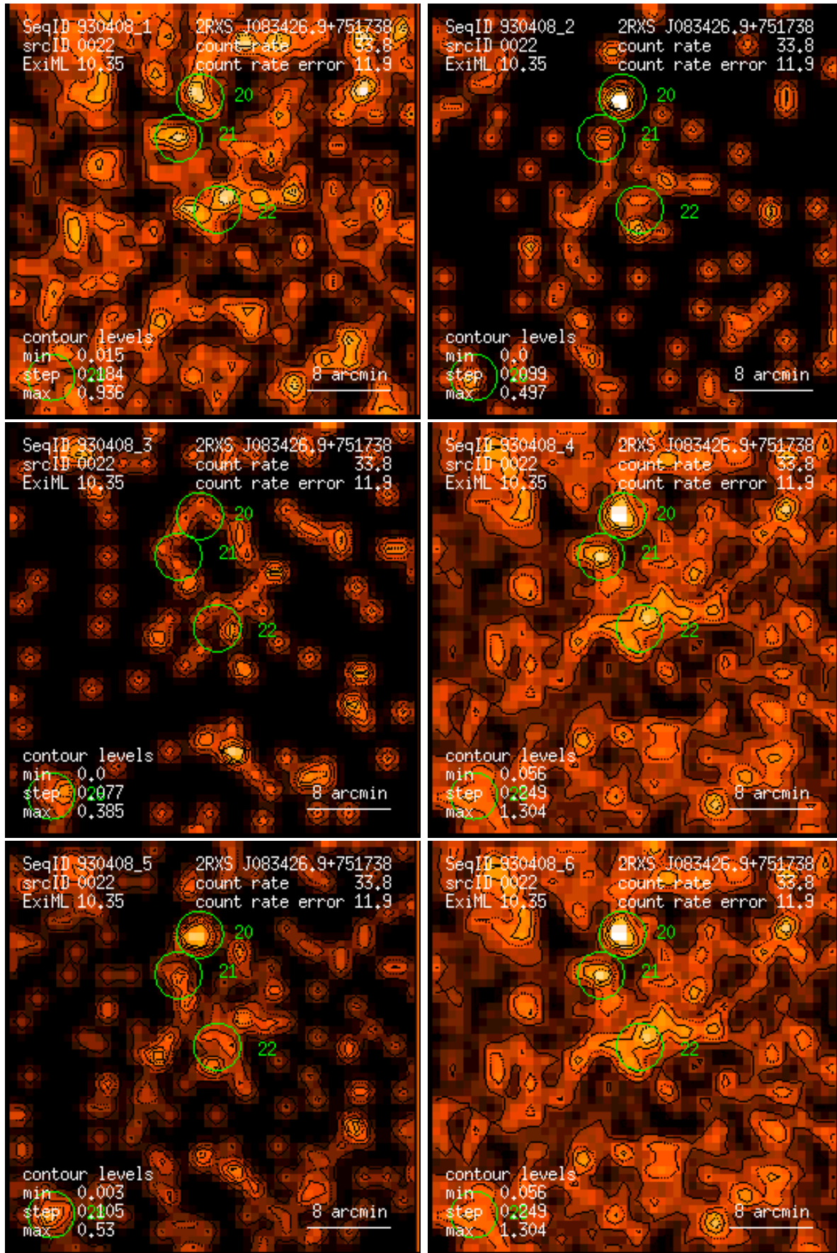
Figure 22: RASS 930408: detection 0022: band rate images, Gaussian filter: (1) PSPC channels 11 – 41, (2) 52 – 90, (3) 91 – 201, (4) 11 – 235, (5) 52 – 201, (6) 11 – 201. Broad band rates in counts/ks. Band rate contour levels in counts/ks/arcmin 2 .
