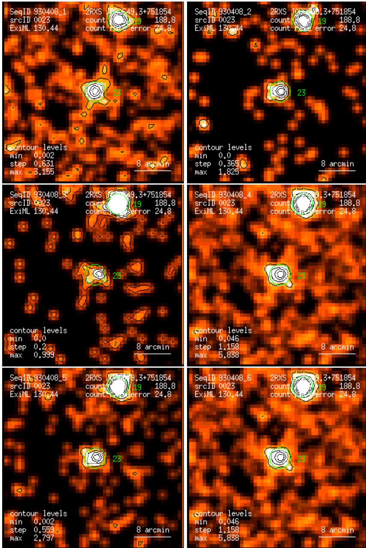
Figure 23: RASS 930408: detection 0023: band rate images, Gaussian filter: (1) PSPC channels 11 – 41, (2) 52 – 90, (3) 91 – 201, (4) 11 – 235, (5) 52 – 201, (6) 11 – 201. Broad band rates in counts/ks. Band rate contour levels in counts/ks/arcmin 2 .
