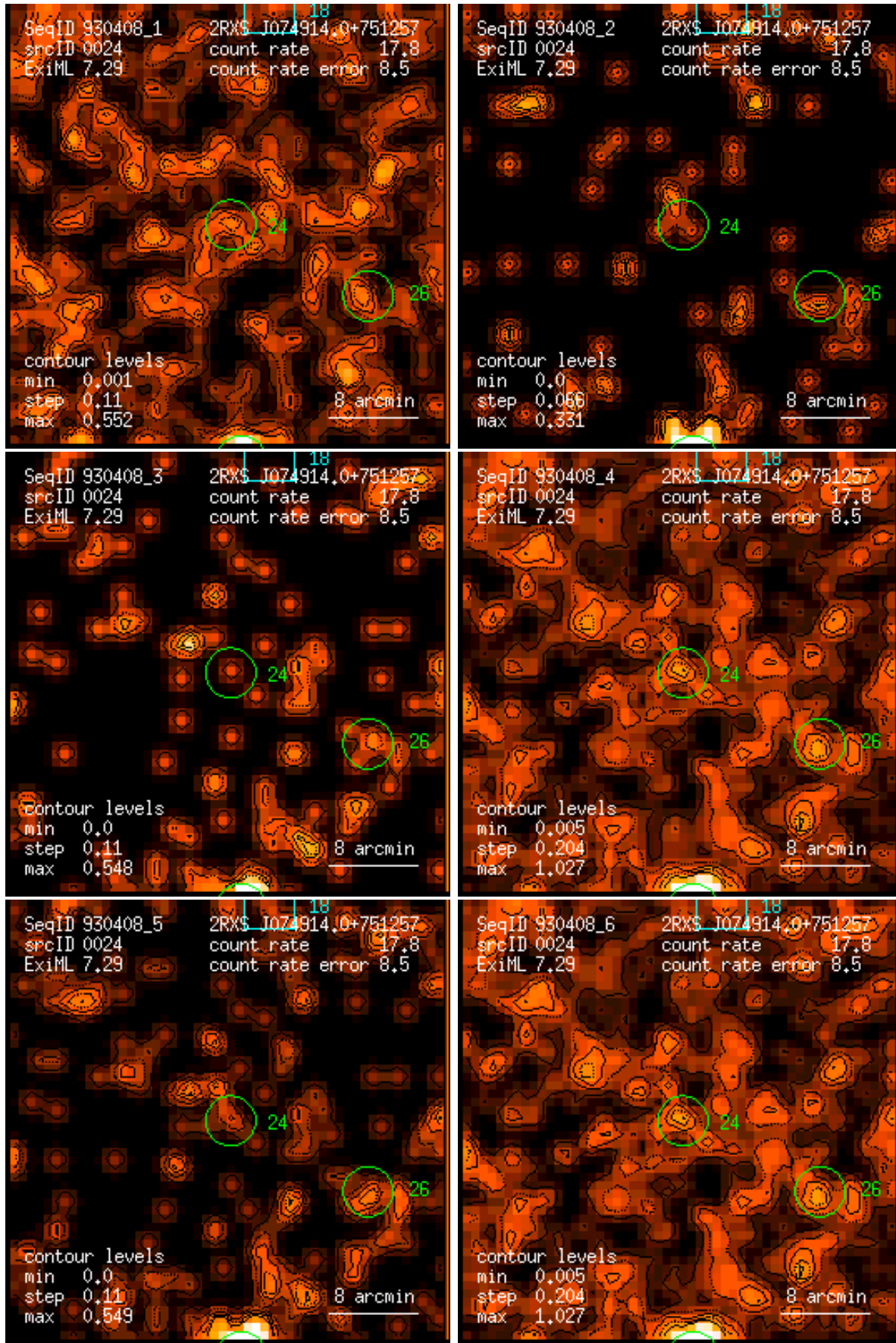
Figure 24: RASS 930408: detection 0024: band rate images, Gaussian filter: (1) PSPC channels 11 – 41, (2) 52 – 90, (3) 91 – 201, (4) 11 – 235, (5) 52 – 201, (6) 11 – 201. Broad band rates in counts/ks. Band rate contour levels in counts/ks/arcmin 2 .
