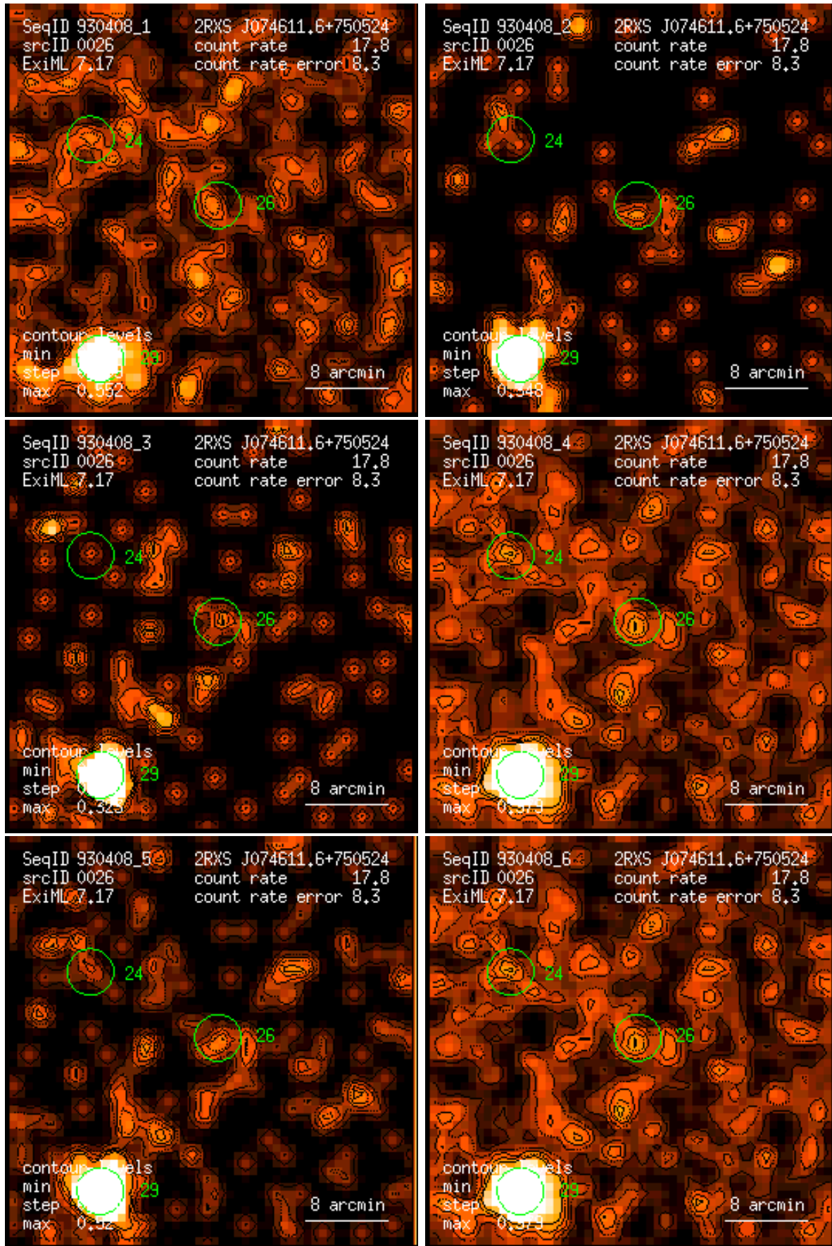
Figure 26: RASS 930408: detection 0026: band rate images, Gaussian filter: (1) PSPC channels 11 – 41, (2) 52 – 90, (3) 91 – 201, (4) 11 – 235, (5) 52 – 201, (6) 11 – 201. Broad band rates in counts/ks. Band rate contour levels in counts/ks/arcmin 2 .
