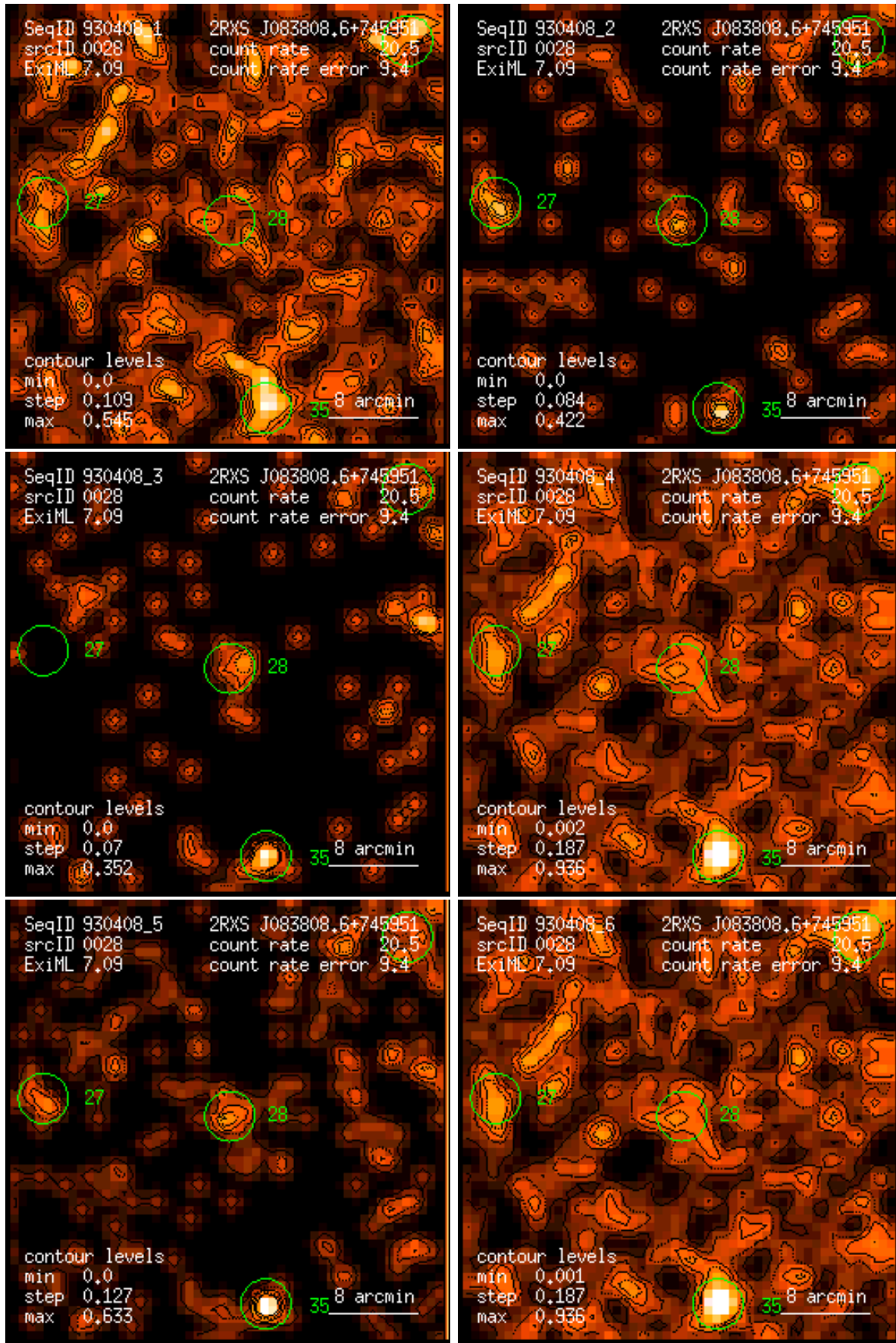
Figure 28: RASS 930408: detection 0028: band rate images, Gaussian filter: (1) PSPC channels 11 – 41, (2) 52 – 90, (3) 91 – 201, (4) 11 – 235, (5) 52 – 201, (6) 11 – 201. Broad band rates in counts/ks. Band rate contour levels in counts/ks/arcmin 2 .
