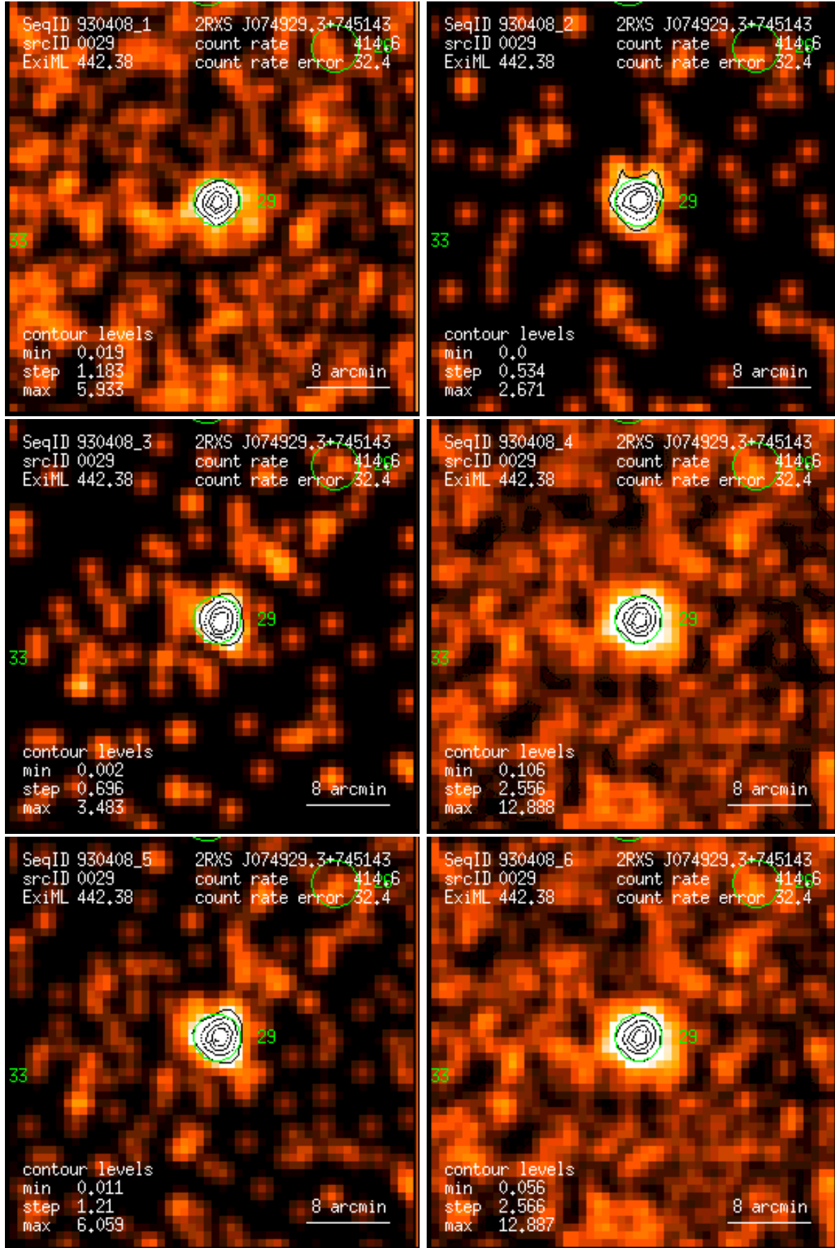
Figure 29: RASS 930408: detection 0029: band rate images, Gaussian filter: (1) PSPC channels 11 – 41, (2) 52 – 90, (3) 91 – 201, (4) 11 – 235, (5) 52 – 201, (6) 11 – 201. Broad band rates in counts/ks. Band rate contour levels in counts/ks/arcmin 2 .
