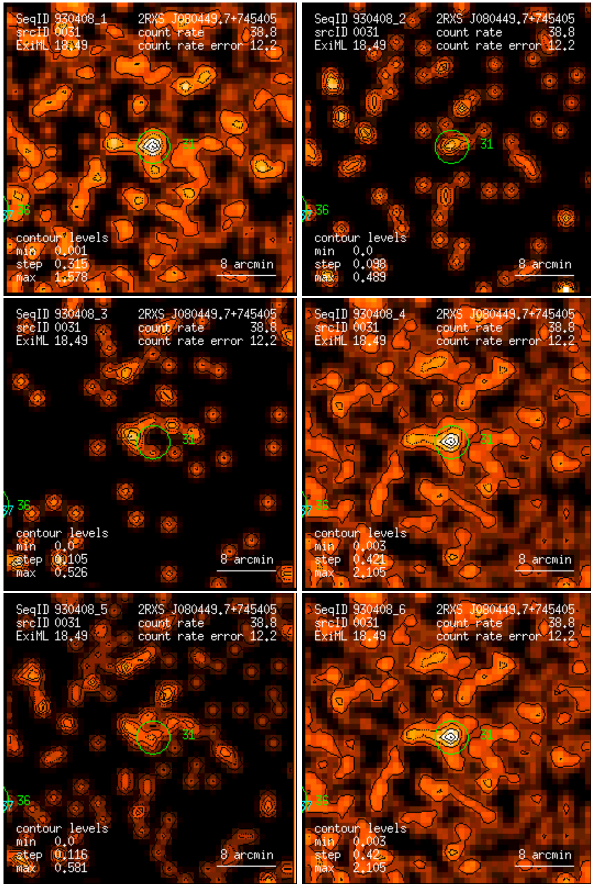
Figure 31: RASS 930408: detection 0031: band rate images, Gaussian filter: (1) PSPC channels 11 – 41, (2) 52 – 90, (3) 91 – 201, (4) 11 – 235, (5) 52 – 201, (6) 11 – 201. Broad band rates in counts/ks. Band rate contour levels in counts/ks/arcmin 2 .
