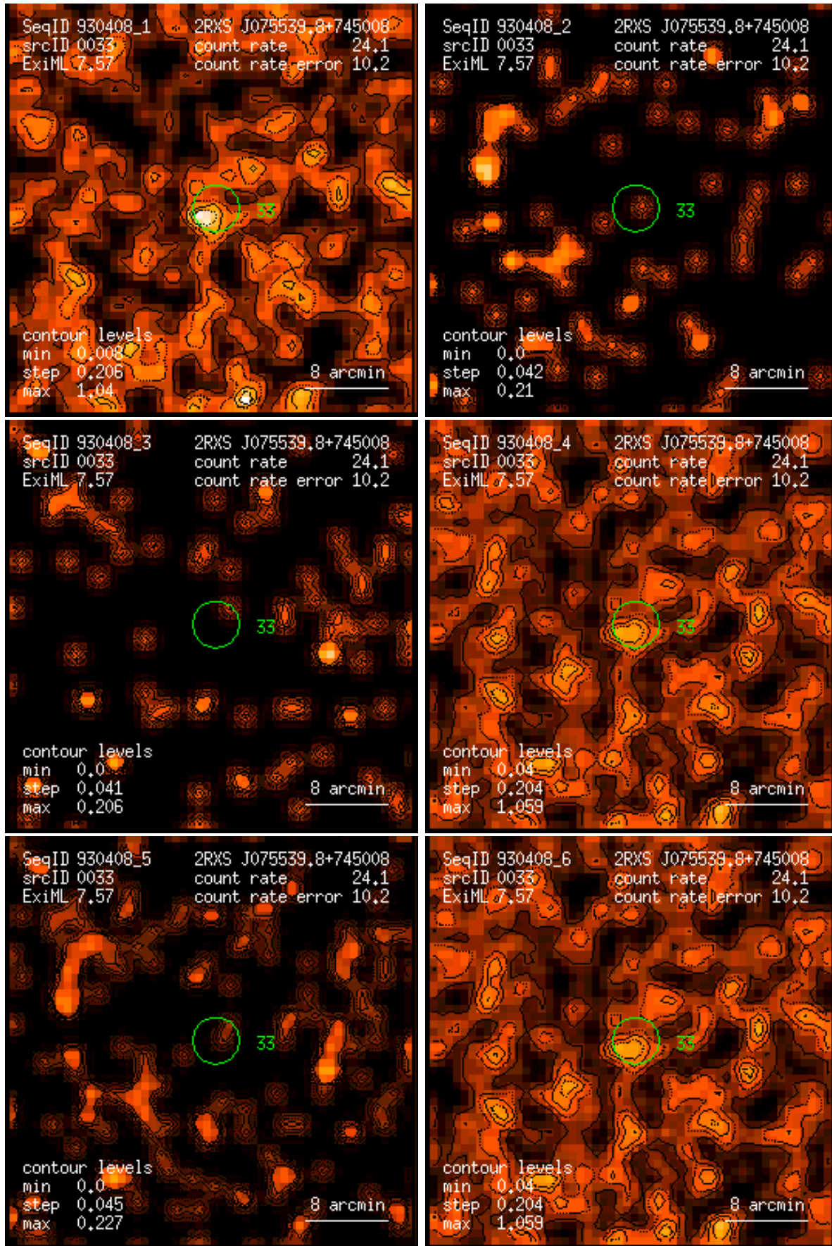
Figure 33: RASS 930408: detection 0033: band rate images, Gaussian filter: (1) PSPC channels 11 – 41, (2) 52 – 90, (3) 91 – 201, (4) 11 – 235, (5) 52 – 201, (6) 11 – 201. Broad band rates in counts/ks. Band rate contour levels in counts/ks/arcmin 2 .
