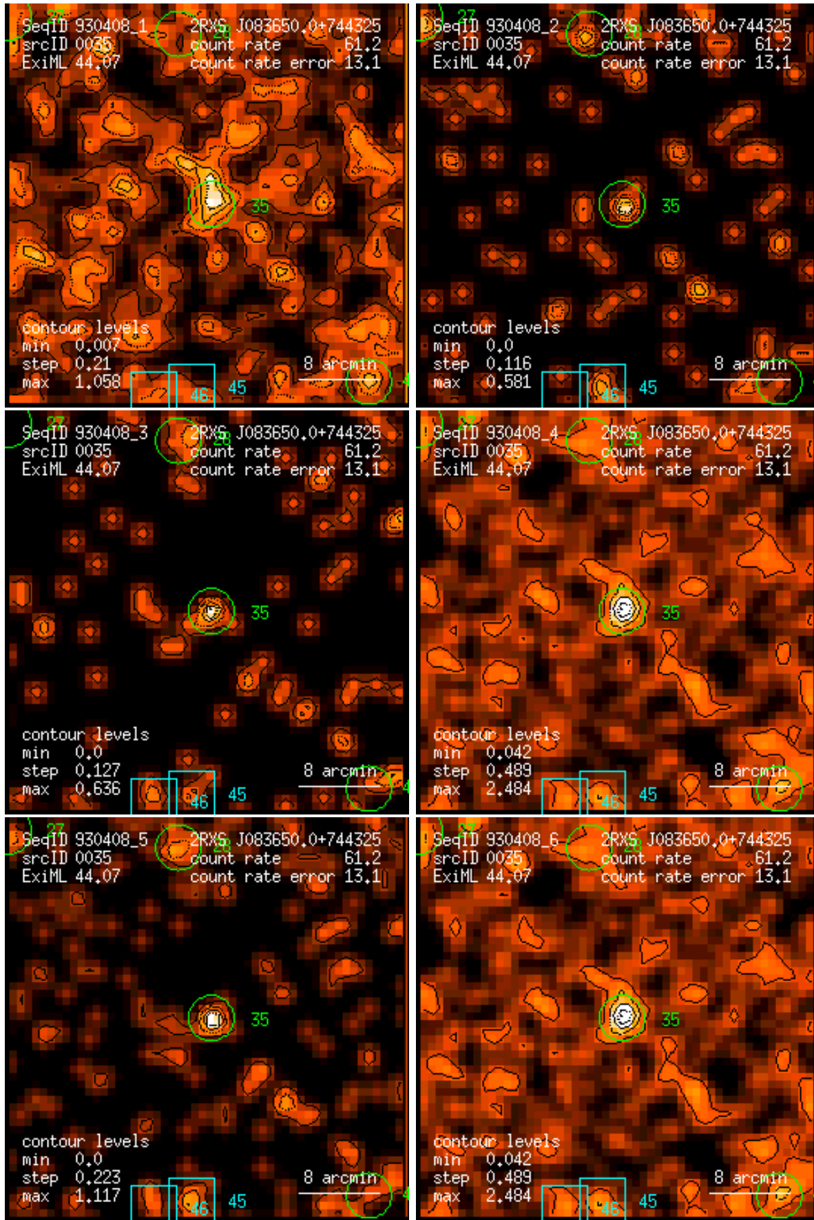
Figure 35: RASS 930408: detection 0035: band rate images, Gaussian filter: (1) PSPC channels 11 – 41, (2) 52 – 90, (3) 91 – 201, (4) 11 – 235, (5) 52 – 201, (6) 11 – 201. Broad band rates in counts/ks. Band rate contour levels in counts/ks/arcmin 2 .
