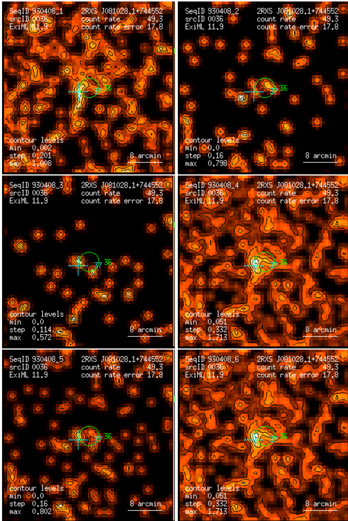
Figure 36: RASS 930408: detection 0036: band rate images, Gaussian filter: (1) PSPC channels 11 – 41, (2) 52 – 90, (3) 91 – 201, (4) 11 – 235, (5) 52 – 201, (6) 11 – 201. Broad band rates in counts/ks. Band rate contour levels in counts/ks/arcmin 2 .
