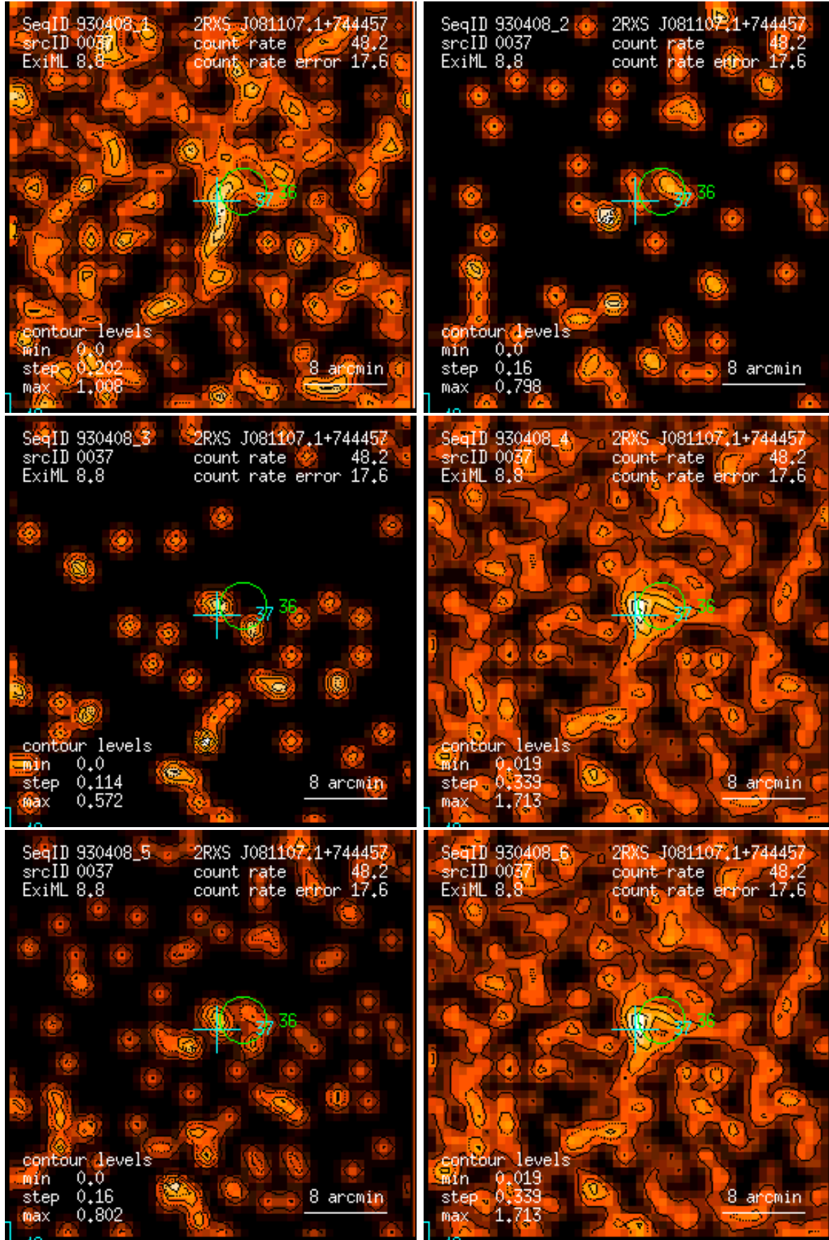
Figure 37: RASS 930408: detection 0037: band rate images, Gaussian filter: (1) PSPC channels 11 – 41, (2) 52 – 90, (3) 91 – 201, (4) 11 – 235, (5) 52 – 201, (6) 11 – 201. Broad band rates in counts/ks. Band rate contour levels in counts/ks/arcmin 2 .
