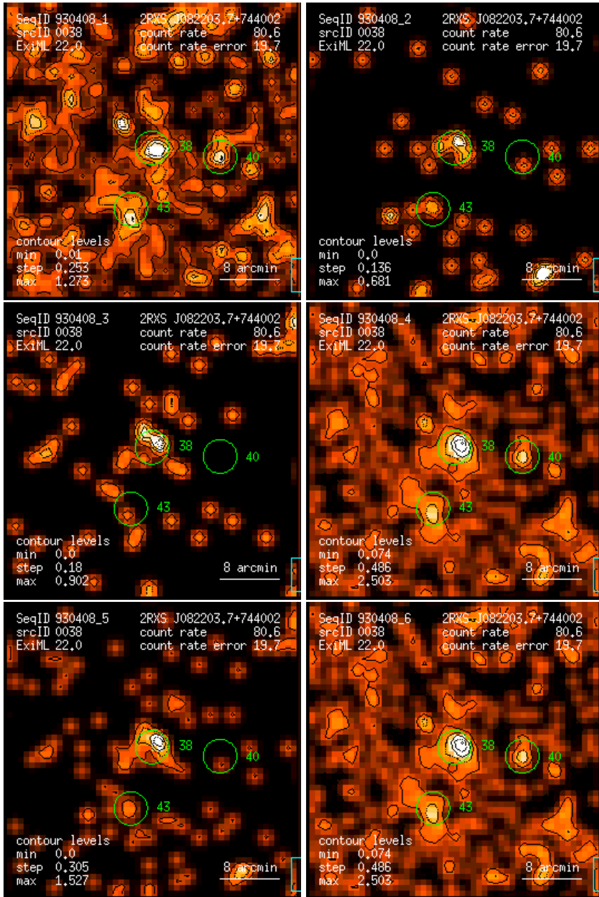
Figure 38: RASS 930408: detection 0038: band rate images, Gaussian filter: (1) PSPC channels 11 – 41, (2) 52 – 90, (3) 91 – 201, (4) 11 – 235, (5) 52 – 201, (6) 11 – 201. Broad band rates in counts/ks. Band rate contour levels in counts/ks/arcmin 2 .
