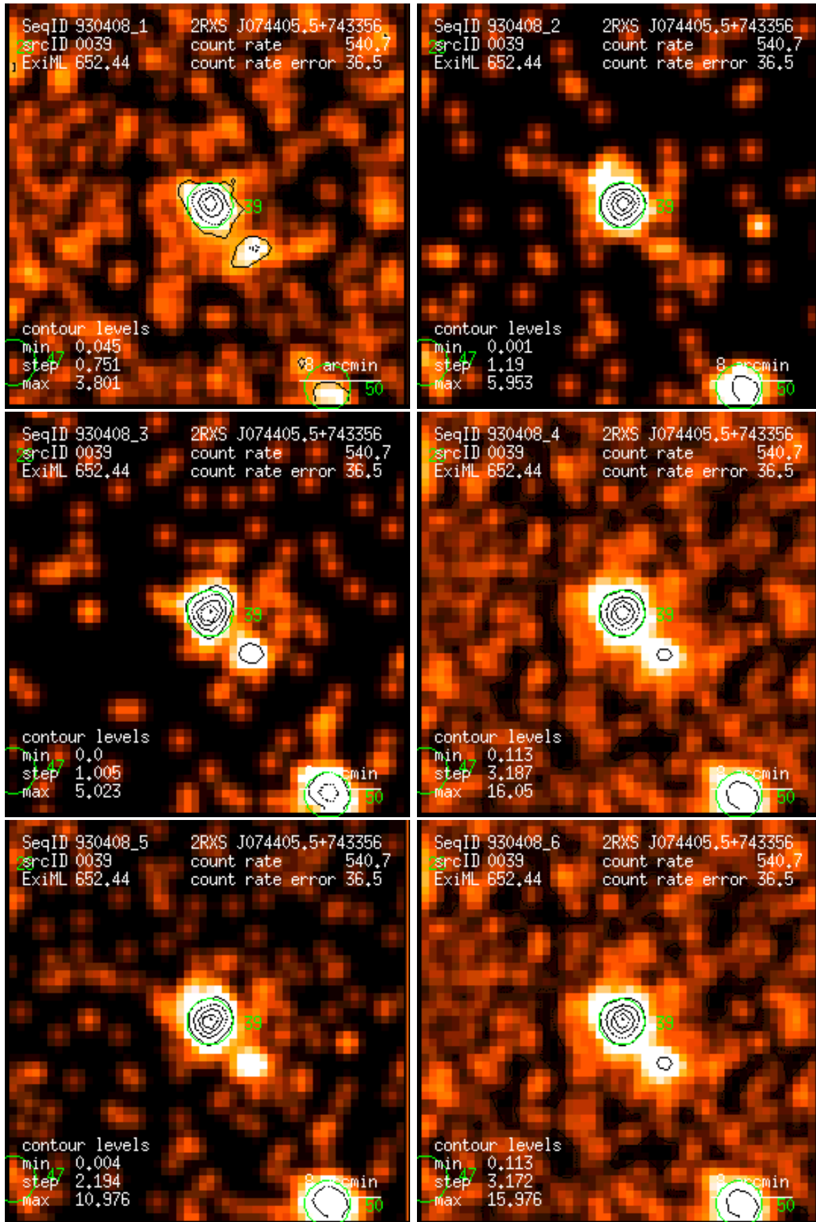
Figure 39: RASS 930408: detection 0039: band rate images, Gaussian filter: (1) PSPC channels 11 – 41, (2) 52 – 90, (3) 91 – 201, (4) 11 – 235, (5) 52 – 201, (6) 11 – 201. Broad band rates in counts/ks. Band rate contour levels in counts/ks/arcmin 2 .
