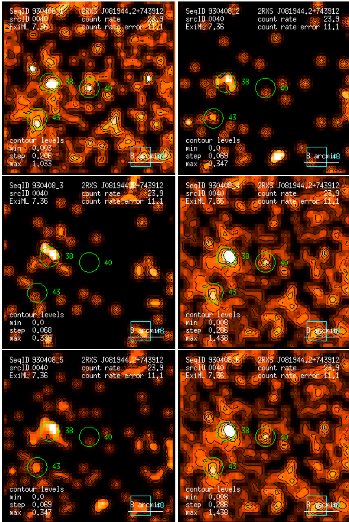
Figure 40: RASS 930408: detection 0040: band rate images, Gaussian filter: (1) PSPC channels 11 – 41, (2) 52 – 90, (3) 91 – 201, (4) 11 – 235, (5) 52 – 201, (6) 11 – 201. Broad band rates in counts/ks. Band rate contour levels in counts/ks/arcmin 2 .
