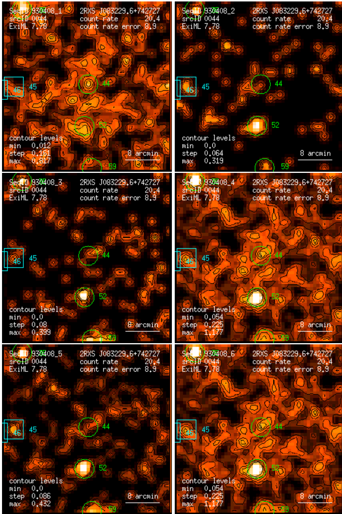
Figure 44: RASS 930408: detection 0044: band rate images, Gaussian filter: (1) PSPC channels 11 – 41, (2) 52 – 90, (3) 91 – 201, (4) 11 – 235, (5) 52 – 201, (6) 11 – 201. Broad band rates in counts/ks. Band rate contour levels in counts/ks/arcmin 2 .
