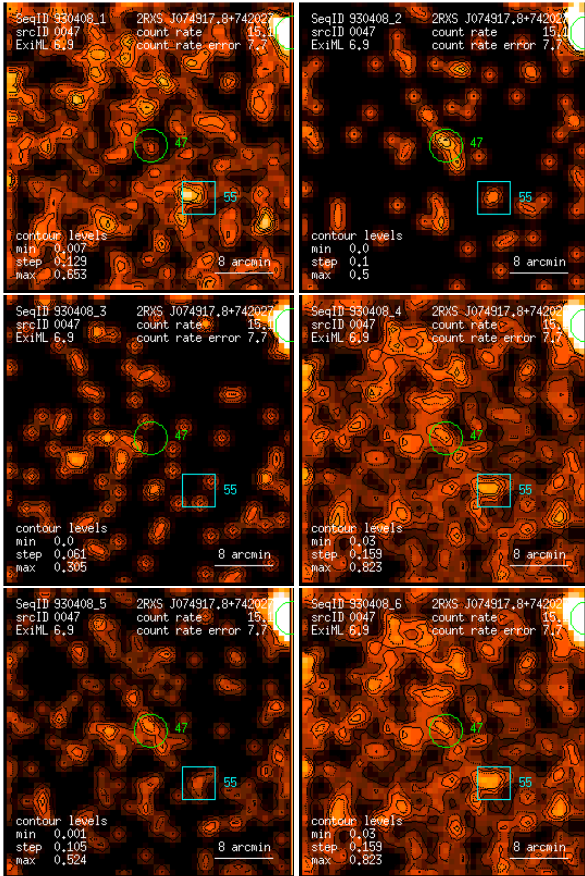
Figure 47: RASS 930408: detection 0047: band rate images, Gaussian filter: (1) PSPC channels 11 – 41, (2) 52 – 90, (3) 91 – 201, (4) 11 – 235, (5) 52 – 201, (6) 11 – 201. Broad band rates in counts/ks. Band rate contour levels in counts/ks/arcmin 2 .
