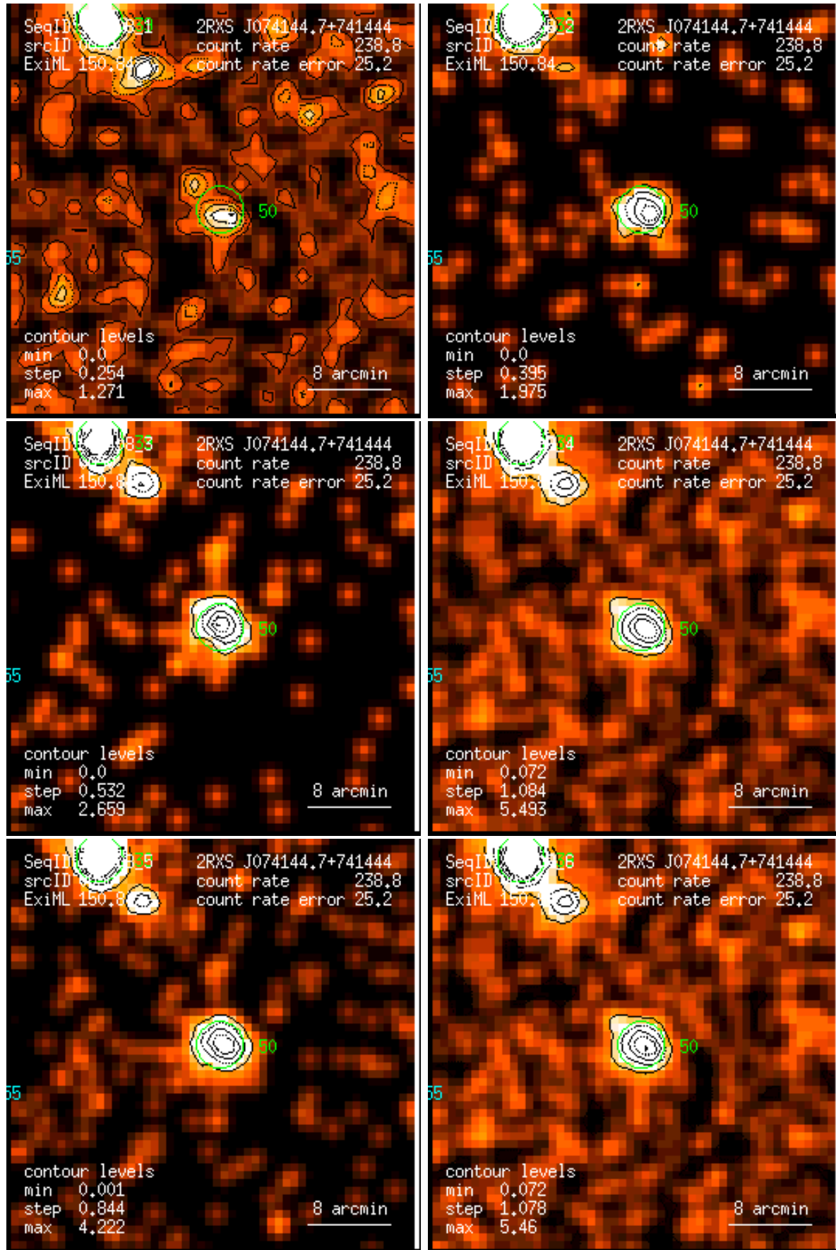
Figure 50: RASS 930408: detection 0050: band rate images, Gaussian filter: (1) PSPC channels 11 – 41, (2) 52 – 90, (3) 91 – 201, (4) 11 – 235, (5) 52 – 201, (6) 11 – 201. Broad band rates in counts/ks. Band rate contour levels in counts/ks/arcmin 2 .
