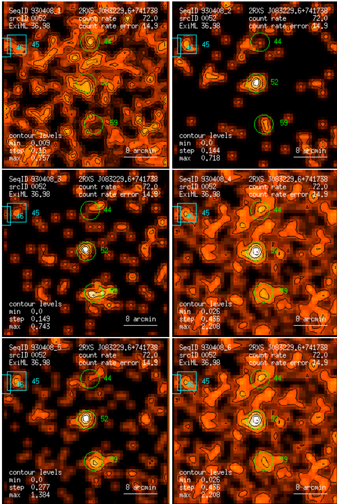
Figure 52: RASS 930408: detection 0052: band rate images, Gaussian filter: (1) PSPC channels 11 – 41, (2) 52 – 90, (3) 91 – 201, (4) 11 – 235, (5) 52 – 201, (6) 11 – 201. Broad band rates in counts/ks. Band rate contour levels in counts/ks/arcmin 2 .
