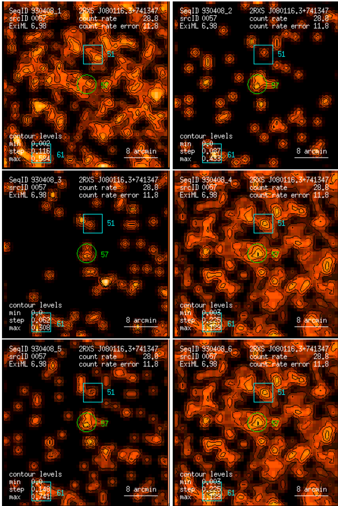
Figure 57: RASS 930408: detection 0057: band rate images, Gaussian filter: (1) PSPC channels 11 – 41, (2) 52 – 90, (3) 91 – 201, (4) 11 – 235, (5) 52 – 201, (6) 11 – 201. Broad band rates in counts/ks. Band rate contour levels in counts/ks/arcmin 2 .
