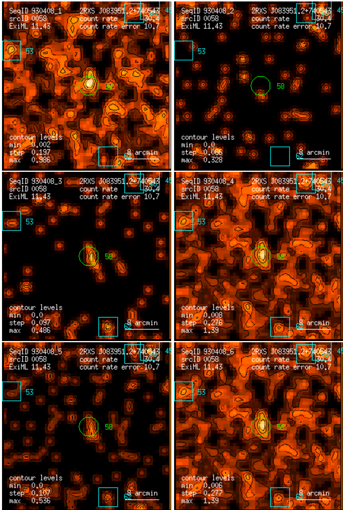
Figure 58: RASS 930408: detection 0058: band rate images, Gaussian filter: (1) PSPC channels 11 – 41, (2) 52 – 90, (3) 91 – 201, (4) 11 – 235, (5) 52 – 201, (6) 11 – 201. Broad band rates in counts/ks. Band rate contour levels in counts/ks/arcmin 2 .
