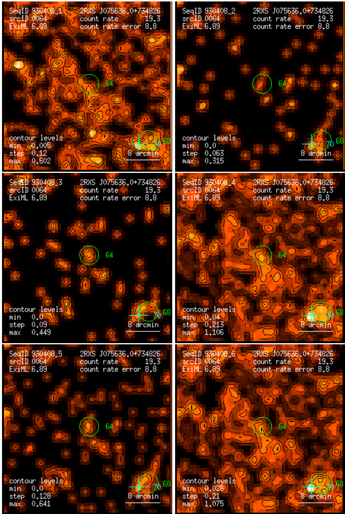
Figure 64: RASS 930408: detection 0064: band rate images, Gaussian filter: (1) PSPC channels 11 – 41, (2) 52 – 90, (3) 91 – 201, (4) 11 – 235, (5) 52 – 201, (6) 11 – 201. Broad band rates in counts/ks. Band rate contour levels in counts/ks/arcmin 2 .
