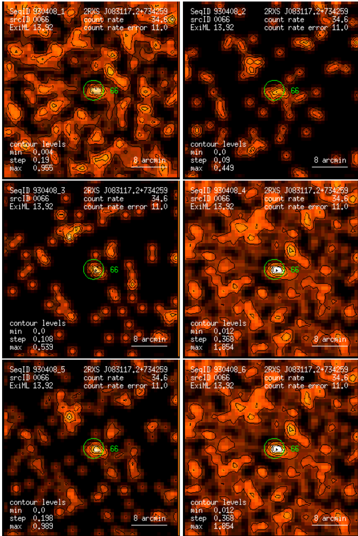
Figure 66: RASS 930408: detection 0066: band rate images, Gaussian filter: (1) PSPC channels 11 – 41, (2) 52 – 90, (3) 91 – 201, (4) 11 – 235, (5) 52 – 201, (6) 11 – 201. Broad band rates in counts/ks. Band rate contour levels in counts/ks/arcmin 2 .
