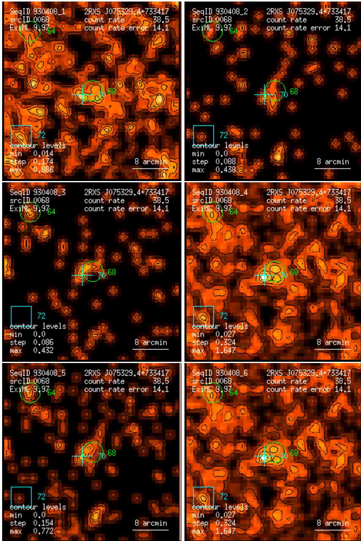
Figure 68: RASS 930408: detection 0068: band rate images, Gaussian filter: (1) PSPC channels 11 – 41, (2) 52 – 90, (3) 91 – 201, (4) 11 – 235, (5) 52 – 201, (6) 11 – 201. Broad band rates in counts/ks. Band rate contour levels in counts/ks/arcmin 2 .
