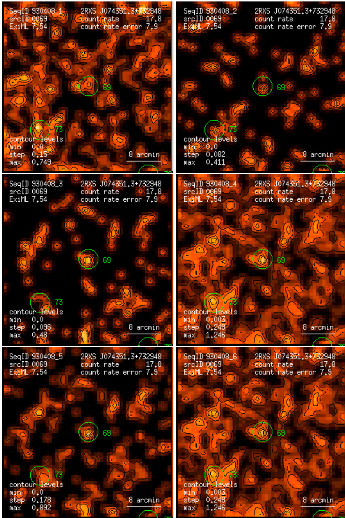
Figure 69: RASS 930408: detection 0069: band rate images, Gaussian filter: (1) PSPC channels 11 – 41, (2) 52 – 90, (3) 91 – 201, (4) 11 – 235, (5) 52 – 201, (6) 11 – 201. Broad band rates in counts/ks. Band rate contour levels in counts/ks/arcmin 2 .
