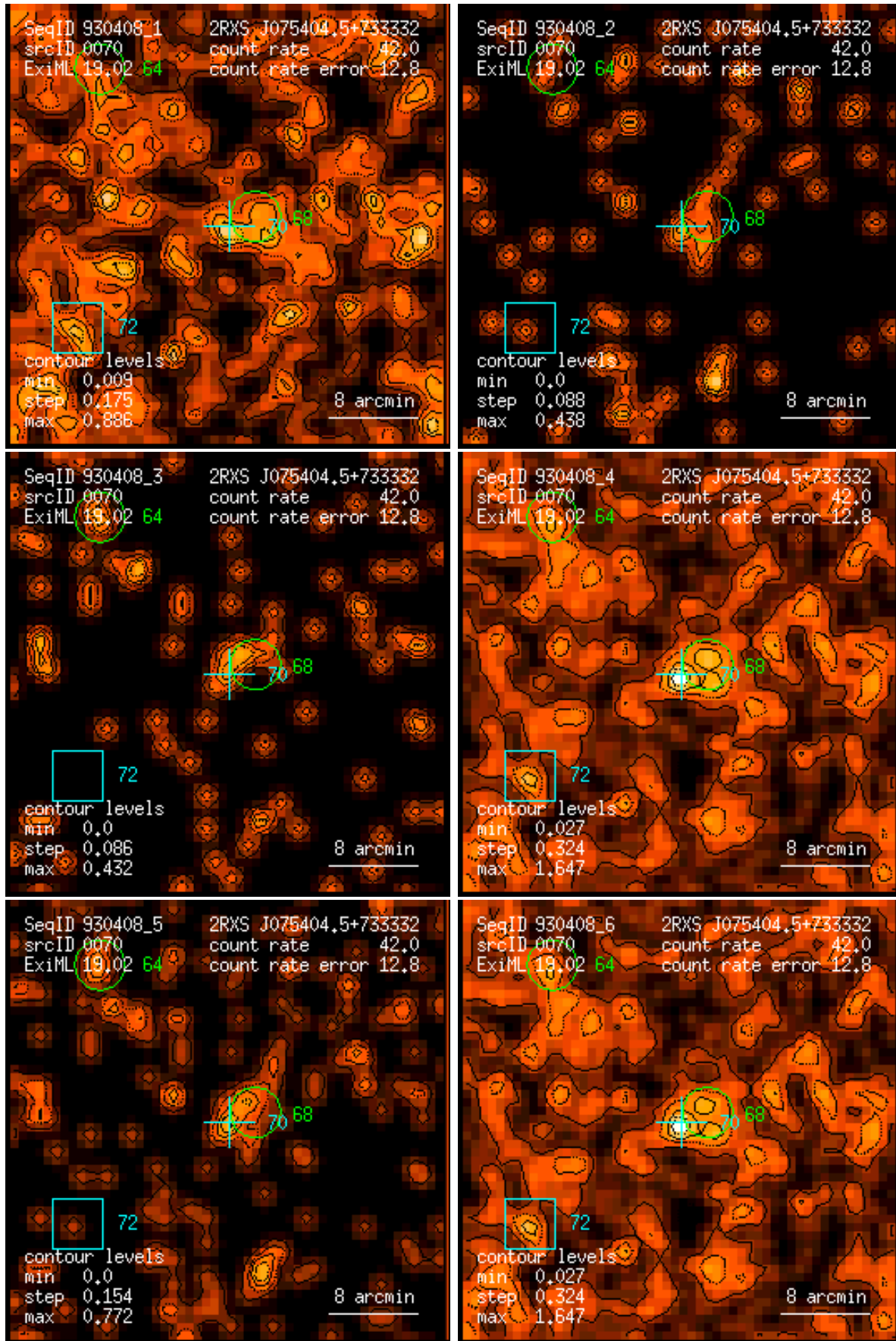
Figure 70: RASS 930408: detection 0070: band rate images, Gaussian filter: (1) PSPC channels 11 – 41, (2) 52 – 90, (3) 91 – 201, (4) 11 – 235, (5) 52 – 201, (6) 11 – 201. Broad band rates in counts/ks. Band rate contour levels in counts/ks/arcmin 2 .
