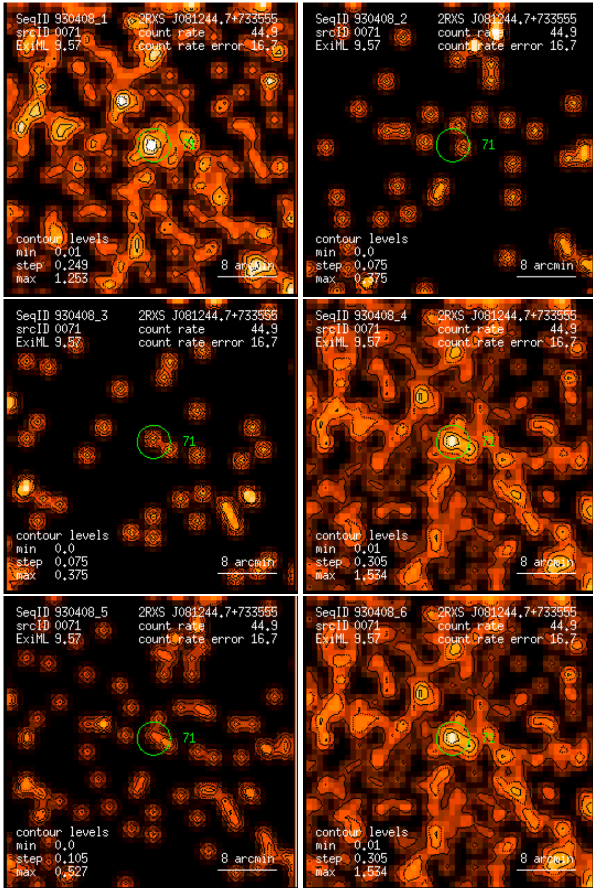
Figure 71: RASS 930408: detection 0071: band rate images, Gaussian filter: (1) PSPC channels 11 – 41, (2) 52 – 90, (3) 91 – 201, (4) 11 – 235, (5) 52 – 201, (6) 11 – 201. Broad band rates in counts/ks. Band rate contour levels in counts/ks/arcmin 2 .
