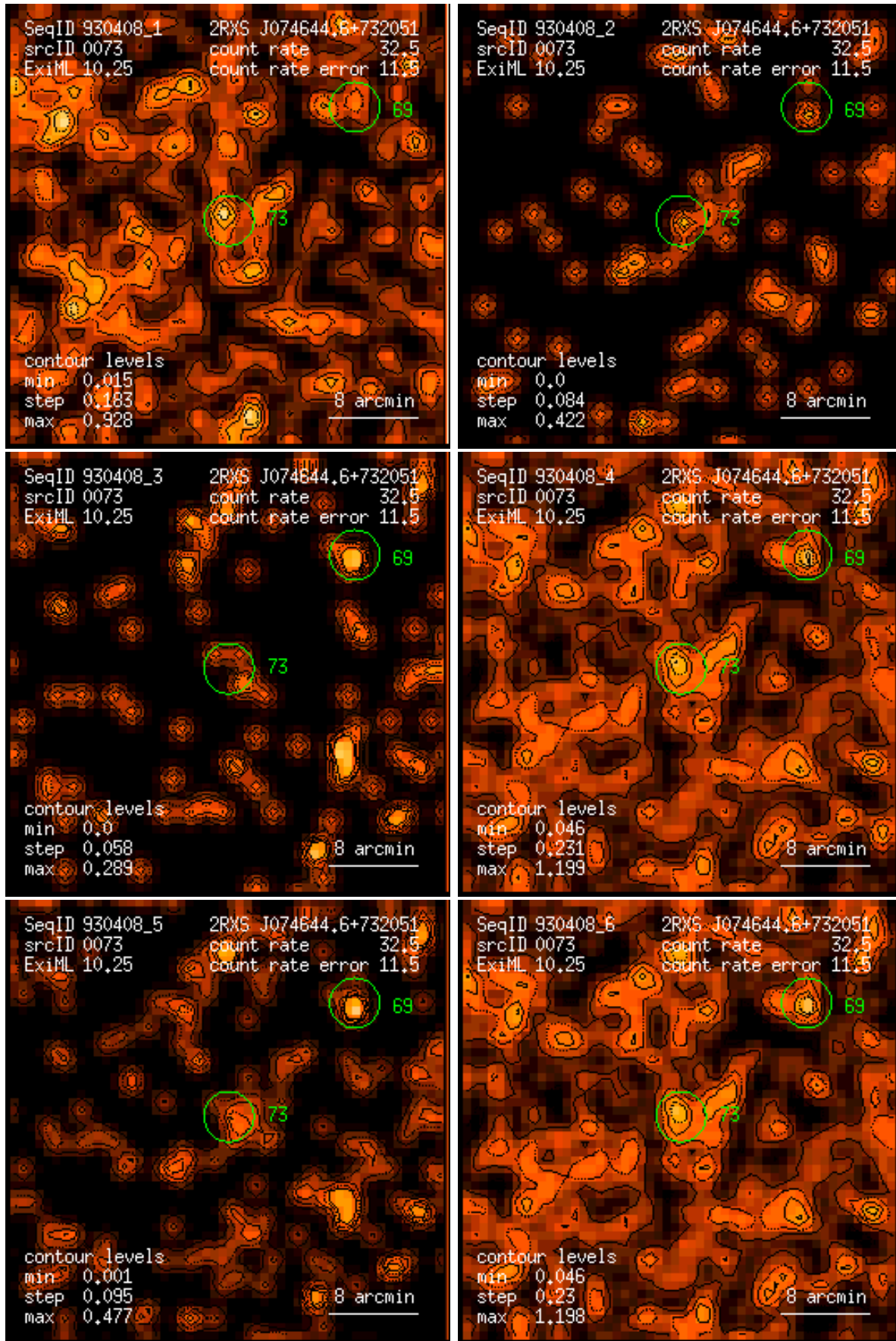
Figure 73: RASS 930408: detection 0073: band rate images, Gaussian filter: (1) PSPC channels 11 – 41, (2) 52 – 90, (3) 91 – 201, (4) 11 – 235, (5) 52 – 201, (6) 11 – 201. Broad band rates in counts/ks. Band rate contour levels in counts/ks/arcmin 2 .
