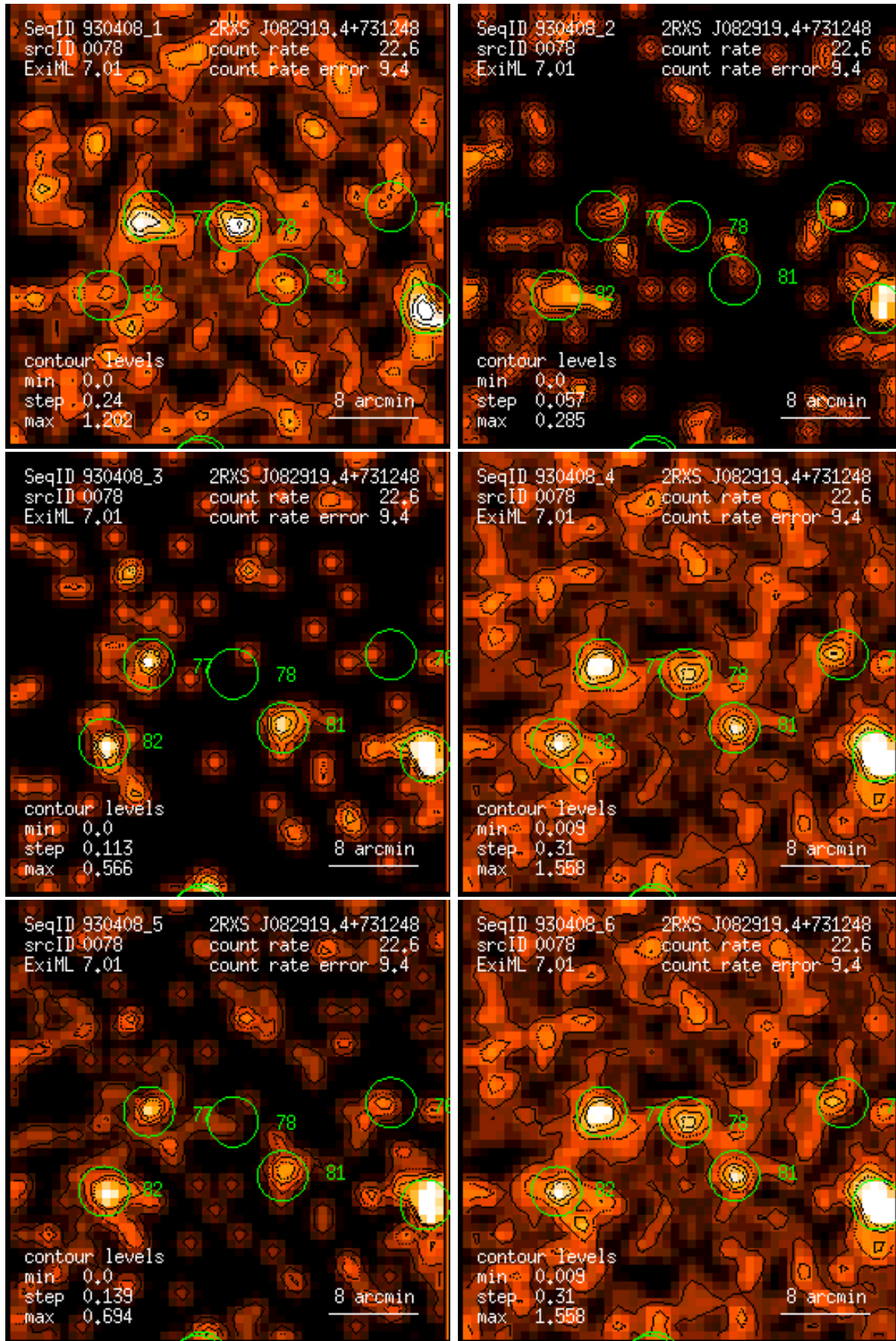
Figure 78: RASS 930408: detection 0078: band rate images, Gaussian filter: (1) PSPC channels 11 – 41, (2) 52 – 90, (3) 91 – 201, (4) 11 – 235, (5) 52 – 201, (6) 11 – 201. Broad band rates in counts/ks. Band rate contour levels in counts/ks/arcmin 2 .
