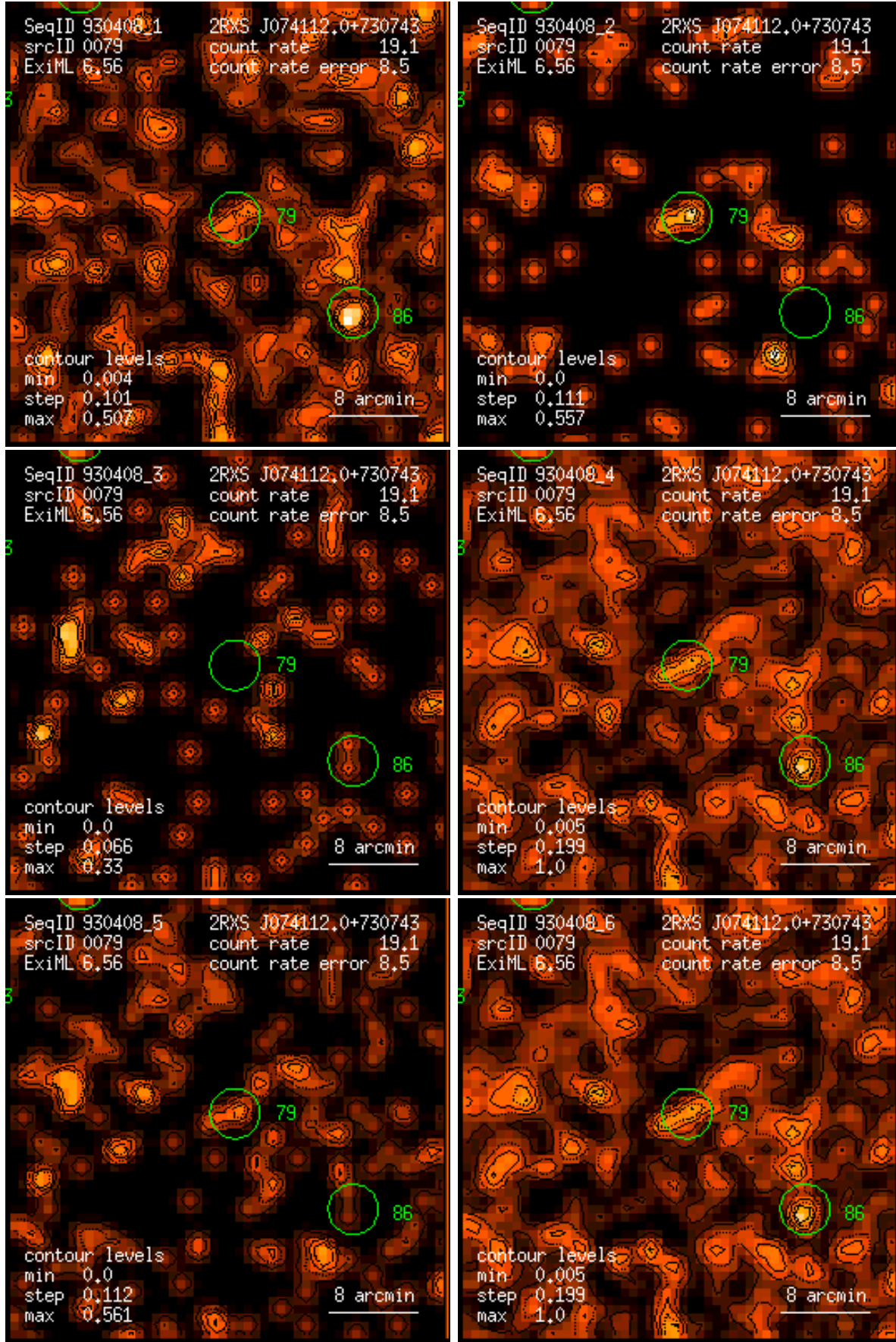
Figure 79: RASS 930408: detection 0079: band rate images, Gaussian filter: (1) PSPC channels 11 – 41, (2) 52 – 90, (3) 91 – 201, (4) 11 – 235, (5) 52 – 201, (6) 11 – 201. Broad band rates in counts/ks. Band rate contour levels in counts/ks/arcmin 2 .
