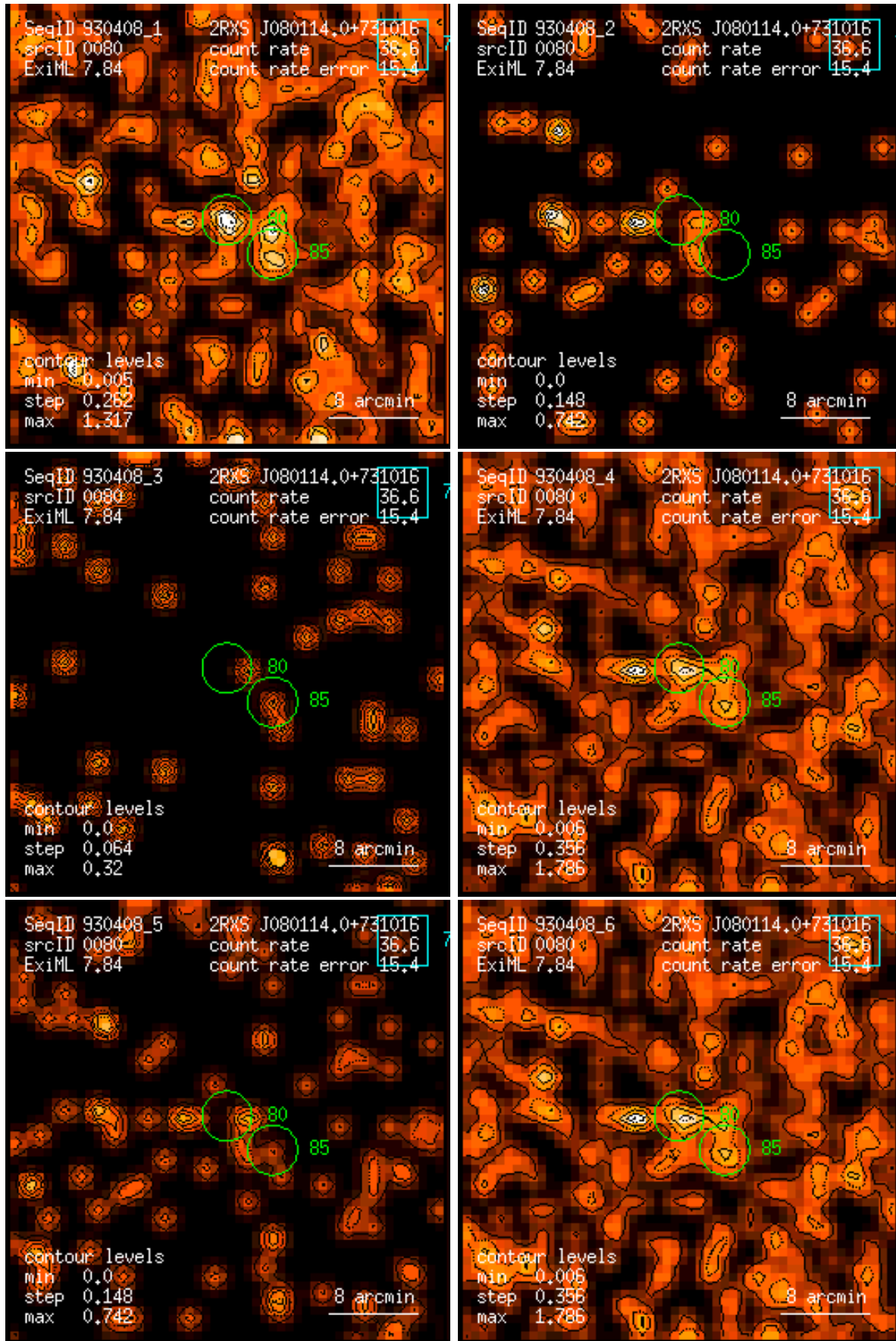
Figure 80: RASS 930408: detection 0080: band rate images, Gaussian filter: (1) PSPC channels 11 – 41, (2) 52 – 90, (3) 91 – 201, (4) 11 – 235, (5) 52 – 201, (6) 11 – 201. Broad band rates in counts/ks. Band rate contour levels in counts/ks/arcmin 2 .
