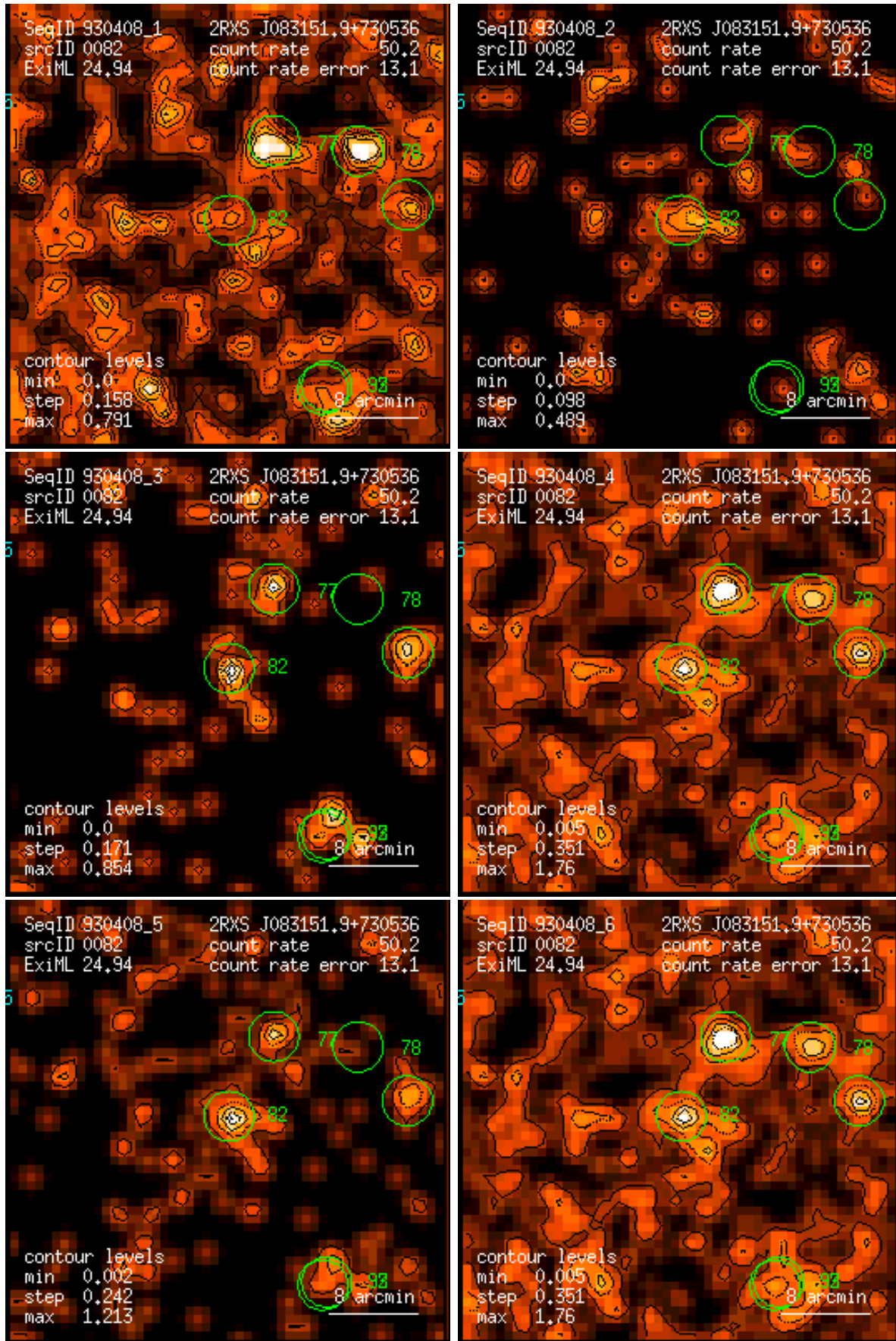
Figure 82: RASS 930408: detection 0082: band rate images, Gaussian filter: (1) PSPC channels 11 – 41, (2) 52 – 90, (3) 91 – 201, (4) 11 – 235, (5) 52 – 201, (6) 11 – 201. Broad band rates in counts/ks. Band rate contour levels in counts/ks/arcmin 2 .
