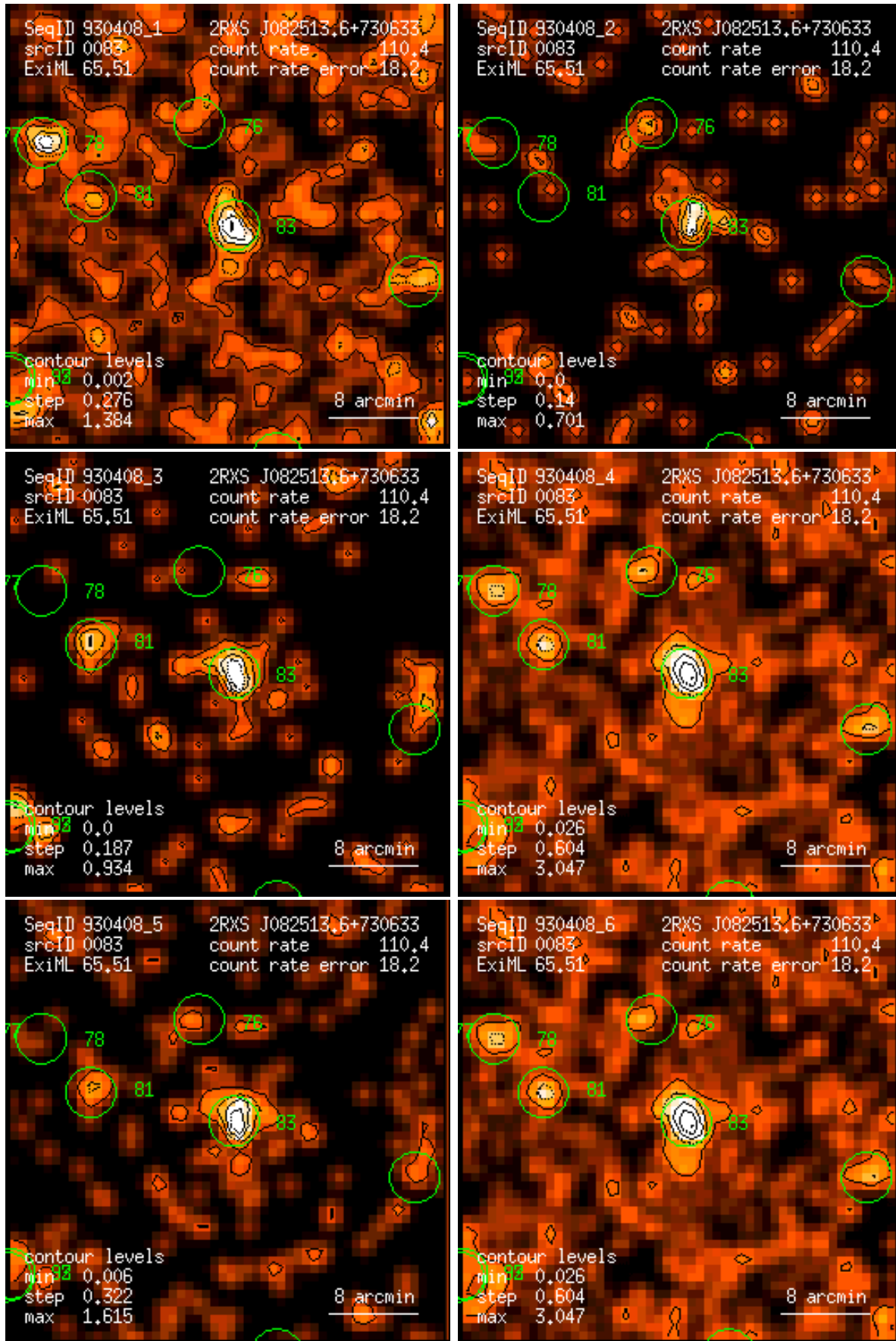
Figure 83: RASS 930408: detection 0083: band rate images, Gaussian filter: (1) PSPC channels 11 – 41, (2) 52 – 90, (3) 91 – 201, (4) 11 – 235, (5) 52 – 201, (6) 11 – 201. Broad band rates in counts/ks. Band rate contour levels in counts/ks/arcmin 2 .
