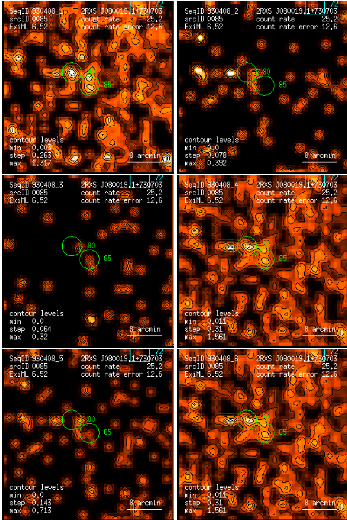
Figure 85: RASS 930408: detection 0085: band rate images, Gaussian filter: (1) PSPC channels 11 – 41, (2) 52 – 90, (3) 91 – 201, (4) 11 – 235, (5) 52 – 201, (6) 11 – 201. Broad band rates in counts/ks. Band rate contour levels in counts/ks/arcmin 2 .
