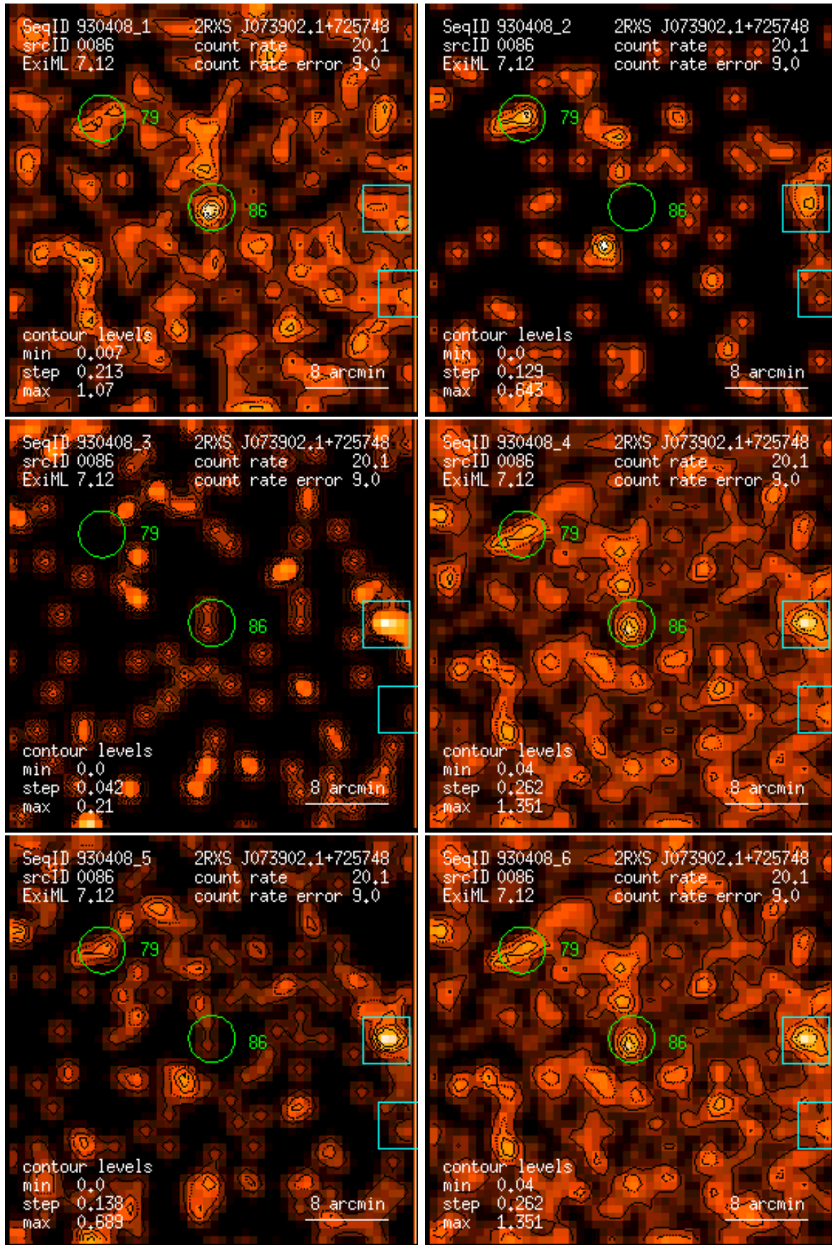
Figure 86: RASS 930408: detection 0086: band rate images, Gaussian filter: (1) PSPC channels 11 – 41, (2) 52 – 90, (3) 91 – 201, (4) 11 – 235, (5) 52 – 201, (6) 11 – 201. Broad band rates in counts/ks. Band rate contour levels in counts/ks/arcmin 2 .
