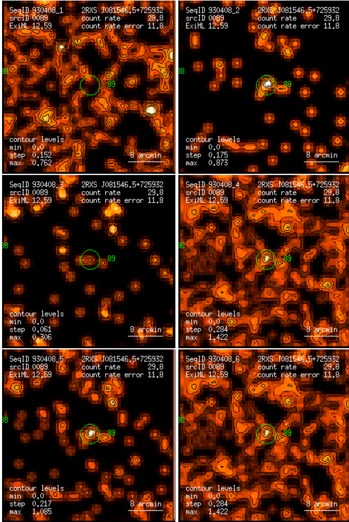
Figure 89: RASS 930408: detection 0089: band rate images, Gaussian filter: (1) PSPC channels 11 – 41, (2) 52 – 90, (3) 91 – 201, (4) 11 – 235, (5) 52 – 201, (6) 11 – 201. Broad band rates in counts/ks. Band rate contour levels in counts/ks/arcmin 2 .
