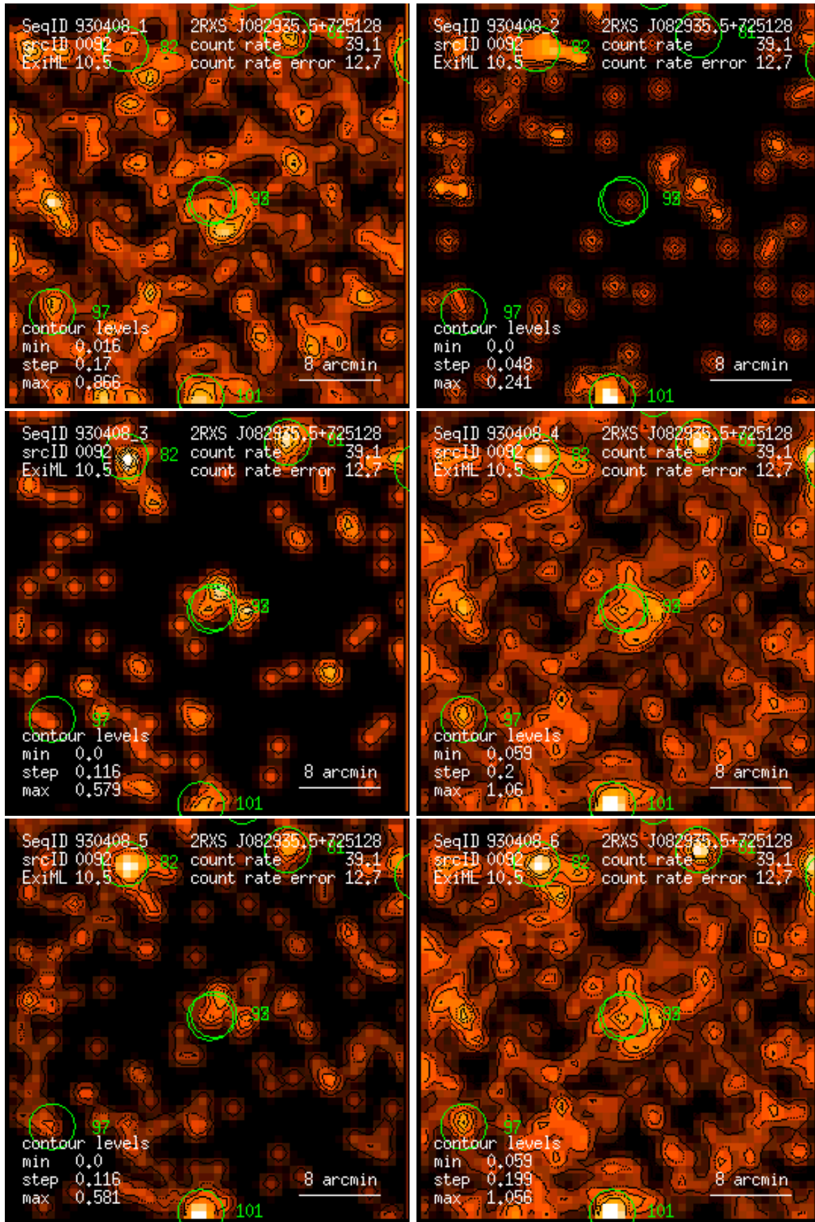
Figure 92: RASS 930408: detection 0092: band rate images, Gaussian filter: (1) PSPC channels 11 – 41, (2) 52 – 90, (3) 91 – 201, (4) 11 – 235, (5) 52 – 201, (6) 11 – 201. Broad band rates in counts/ks. Band rate contour levels in counts/ks/arcmin 2 .
