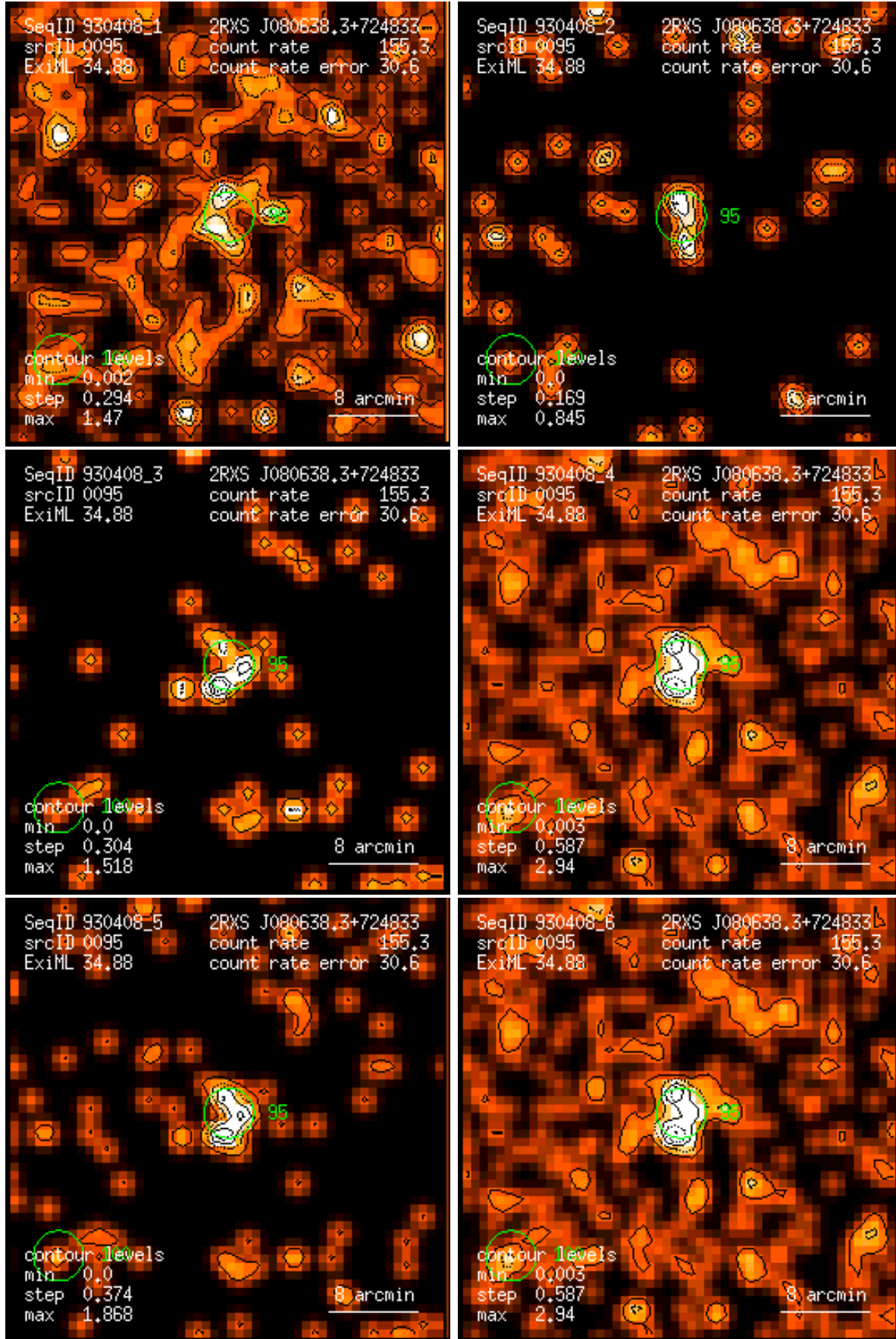
Figure 95: RASS 930408: detection 0095: band rate images, Gaussian filter: (1) PSPC channels 11 – 41, (2) 52 – 90, (3) 91 – 201, (4) 11 – 235, (5) 52 – 201, (6) 11 – 201. Broad band rates in counts/ks. Band rate contour levels in counts/ks/arcmin 2 .
