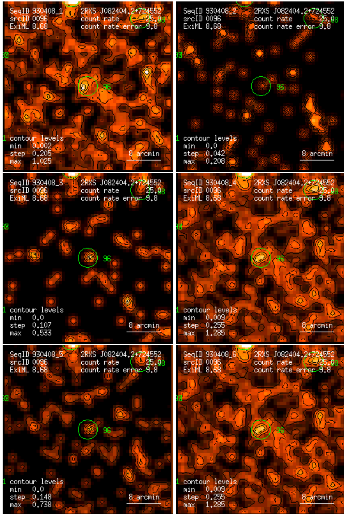
Figure 96: RASS 930408: detection 0096: band rate images, Gaussian filter: (1) PSPC channels 11 – 41, (2) 52 – 90, (3) 91 – 201, (4) 11 – 235, (5) 52 – 201, (6) 11 – 201. Broad band rates in counts/ks. Band rate contour levels in counts/ks/arcmin 2 .
