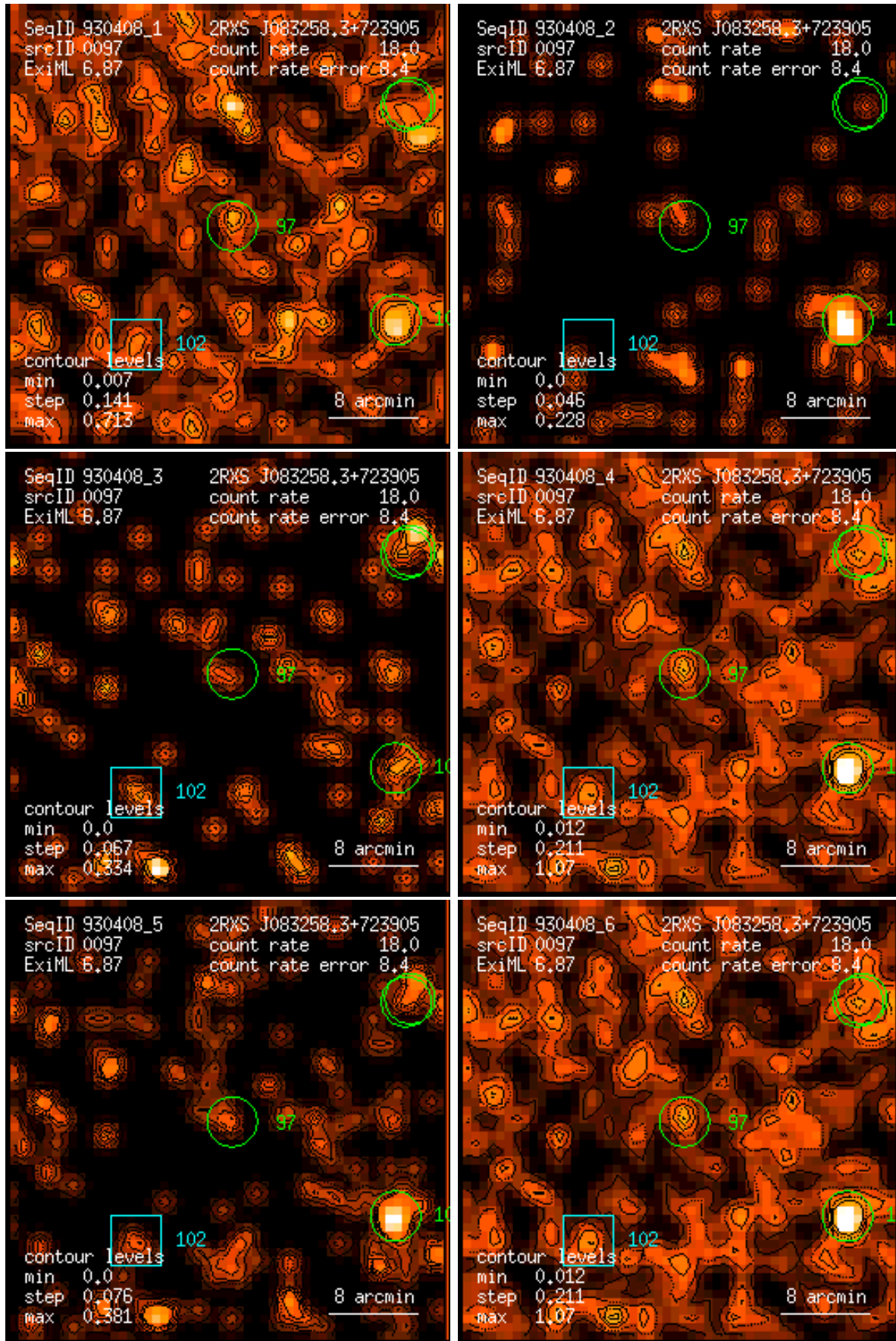
Figure 97: RASS 930408: detection 0097: band rate images, Gaussian filter: (1) PSPC channels 11 – 41, (2) 52 – 90, (3) 91 – 201, (4) 11 – 235, (5) 52 – 201, (6) 11 – 201. Broad band rates in counts/ks. Band rate contour levels in counts/ks/arcmin 2 .
