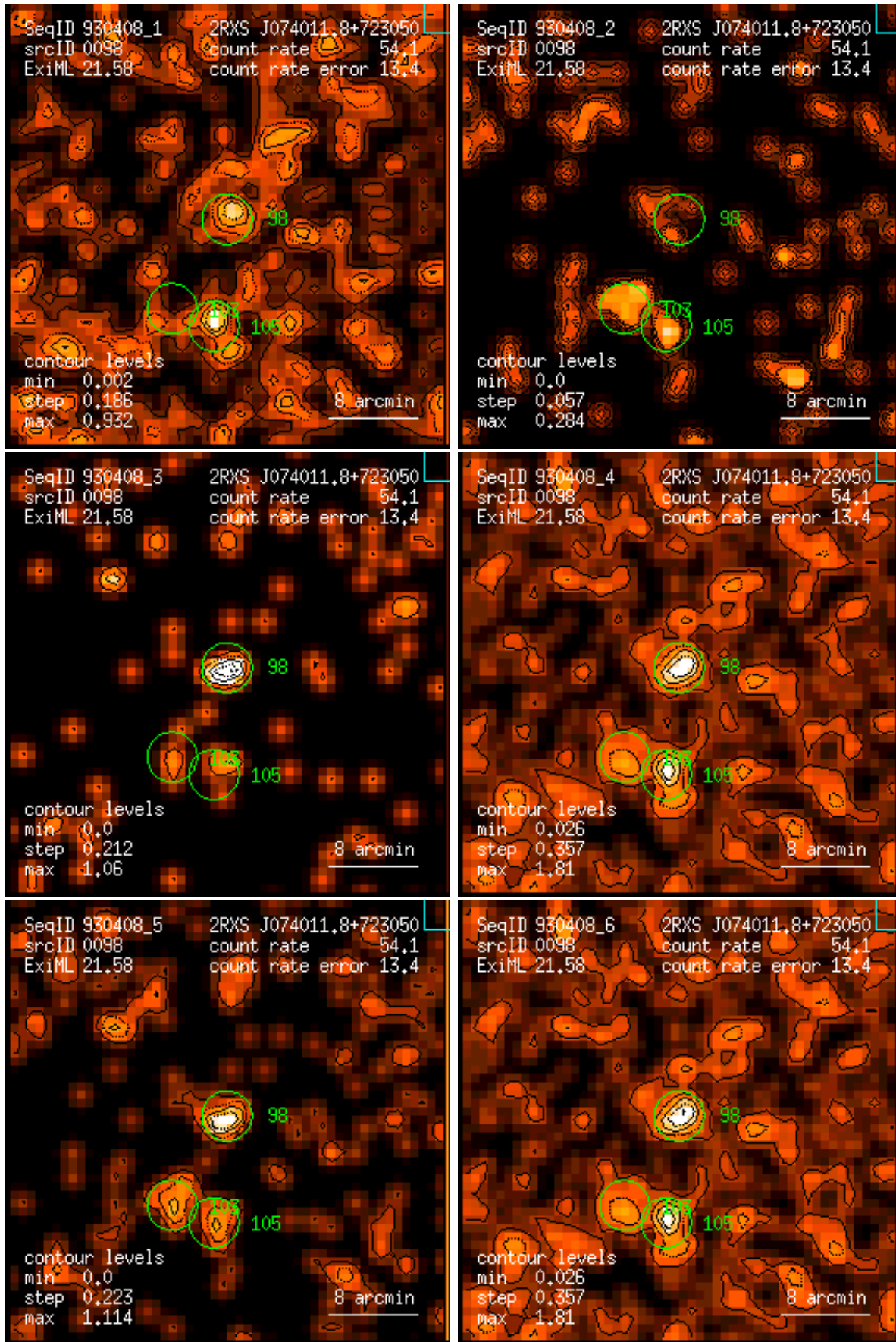
Figure 98: RASS 930408: detection 0098: band rate images, Gaussian filter: (1) PSPC channels 11 – 41, (2) 52 – 90, (3) 91 – 201, (4) 11 – 235, (5) 52 – 201, (6) 11 – 201. Broad band rates in counts/ks. Band rate contour levels in counts/ks/arcmin 2 .
