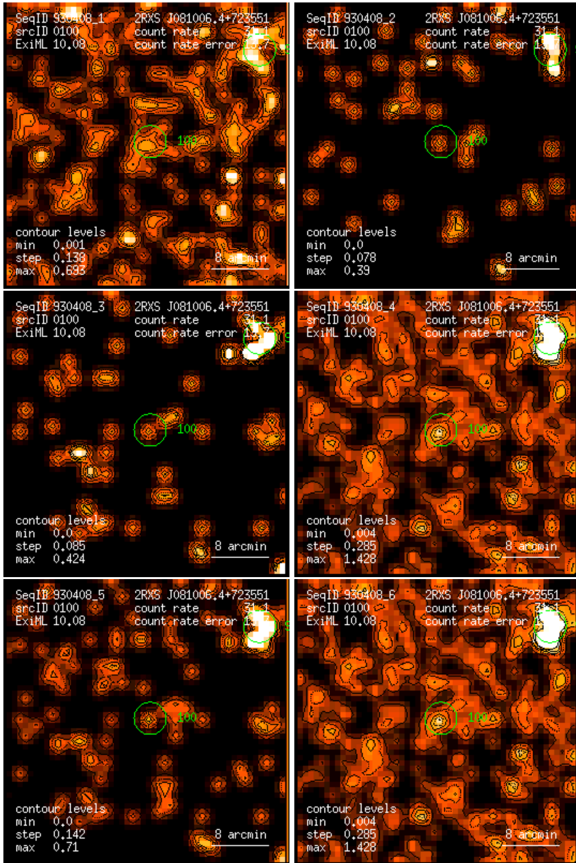
Figure 100: RASS 930408: detection 0100: band rate images, Gaussian filter: (1) PSPC channels 11 – 41, (2) 52 – 90, (3) 91 – 201, (4) 11 – 235, (5) 52 – 201, (6) 11 – 201. Broad band rates in counts/ks. Band rate contour levels in counts/ks/arcmin 2 .
