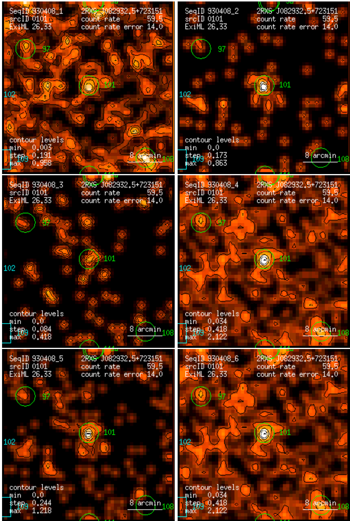
Figure 101: RASS 930408: detection 0101: band rate images, Gaussian filter: (1) PSPC channels 11 – 41, (2) 52 – 90, (3) 91 – 201, (4) 11 – 235, (5) 52 – 201, (6) 11 – 201. Broad band rates in counts/ks. Band rate contour levels in counts/ks/arcmin 2 .
