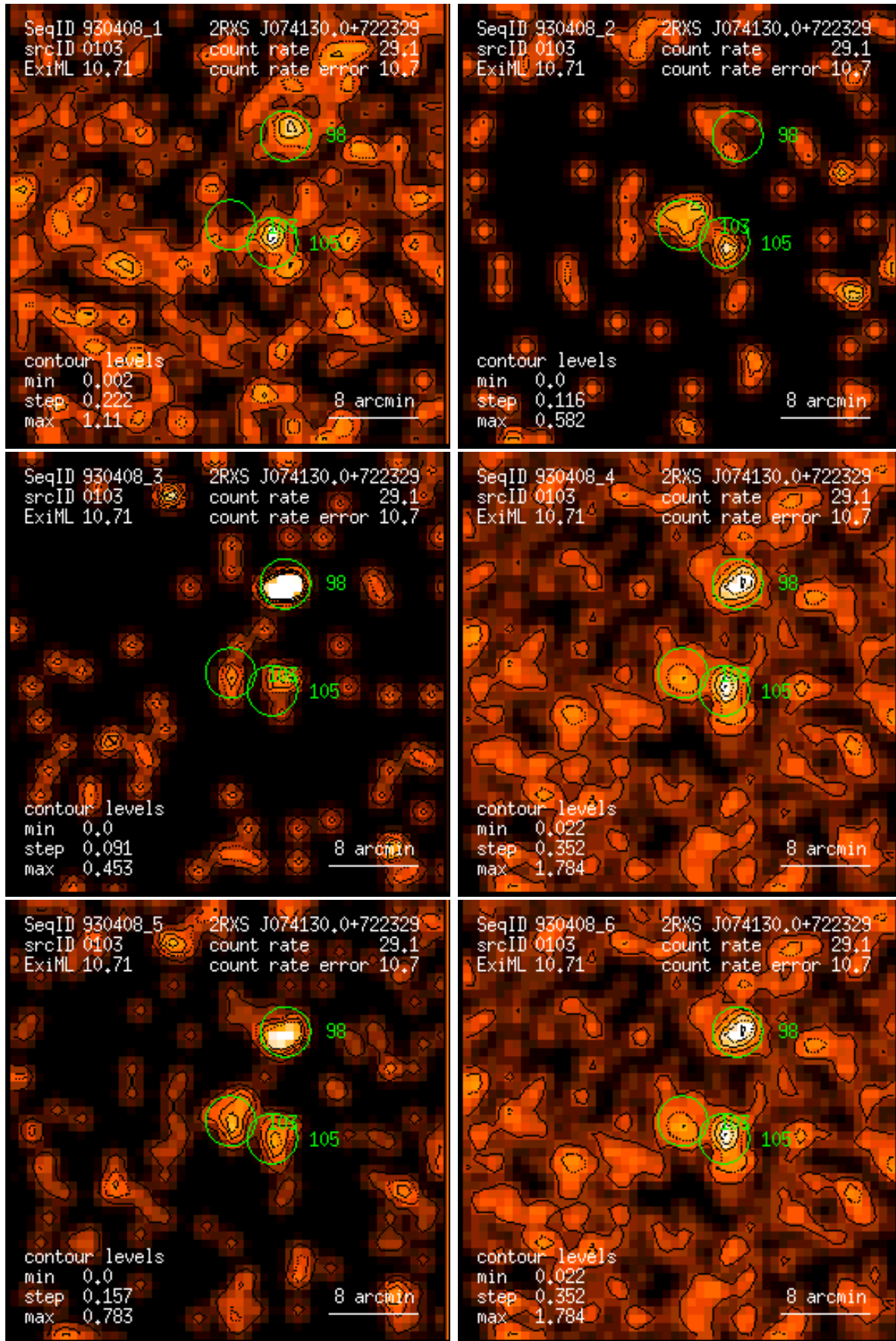
Figure 103: RASS 930408: detection 0103: band rate images, Gaussian filter: (1) PSPC channels 11 – 41, (2) 52 – 90, (3) 91 – 201, (4) 11 – 235, (5) 52 – 201, (6) 11 – 201. Broad band rates in counts/ks. Band rate contour levels in counts/ks/arcmin 2 .
